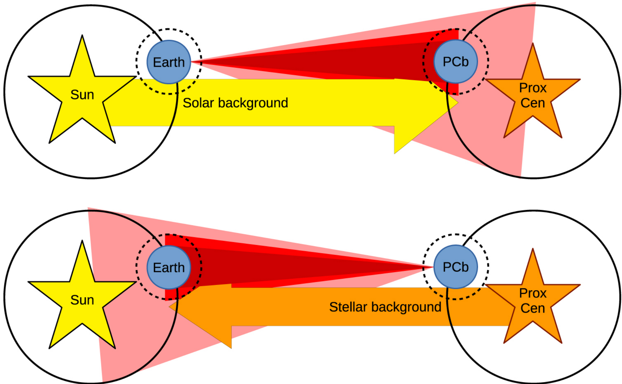
Figure 3. from Optical Detection of Lasers with Near-term Technology at Interstellar Distances null 2018 APJ 867 97 doi:10.3847/1538-4357/aae380 https://dx.doi.org/10.3847/1538-4357/aae380 © 2018. The American Astronomical Society.
