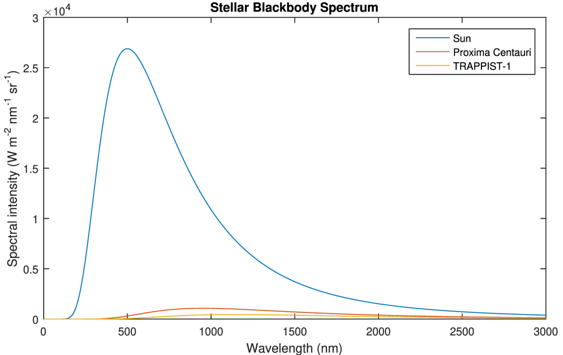
Figure 2. from Optical Detection of Lasers with Near-term Technology at Interstellar Distances null 2018 APJ 867 97 doi:10.3847/1538-4357/aae380 https://dx.doi.org/10.3847/1538-4357/aae380 © 2018. The American Astronomical Society.
