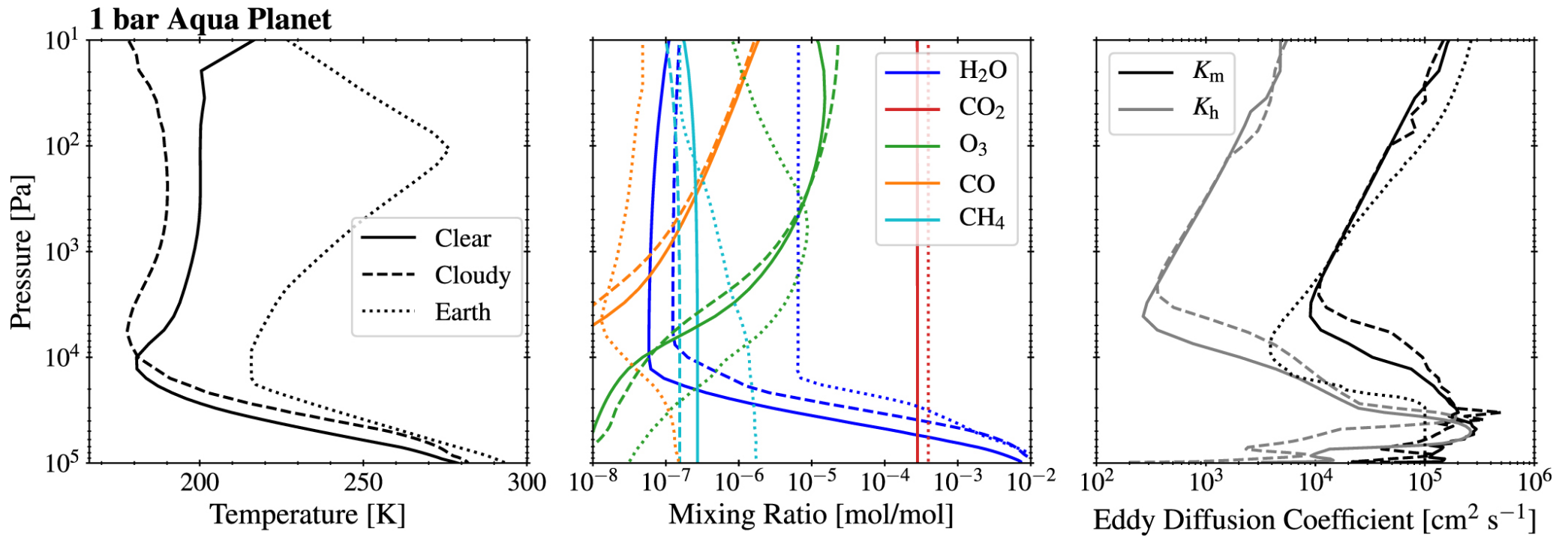
Figure 8. from Evolved Climates and Observational Discriminants for the TRAPPIST-1 Planetary System null 2018 APJ 867 76 doi:10.3847/1538-4357/aae36a https://dx.doi.org/10.3847/1538-4357/aae36a © 2018. The American Astronomical Society.
