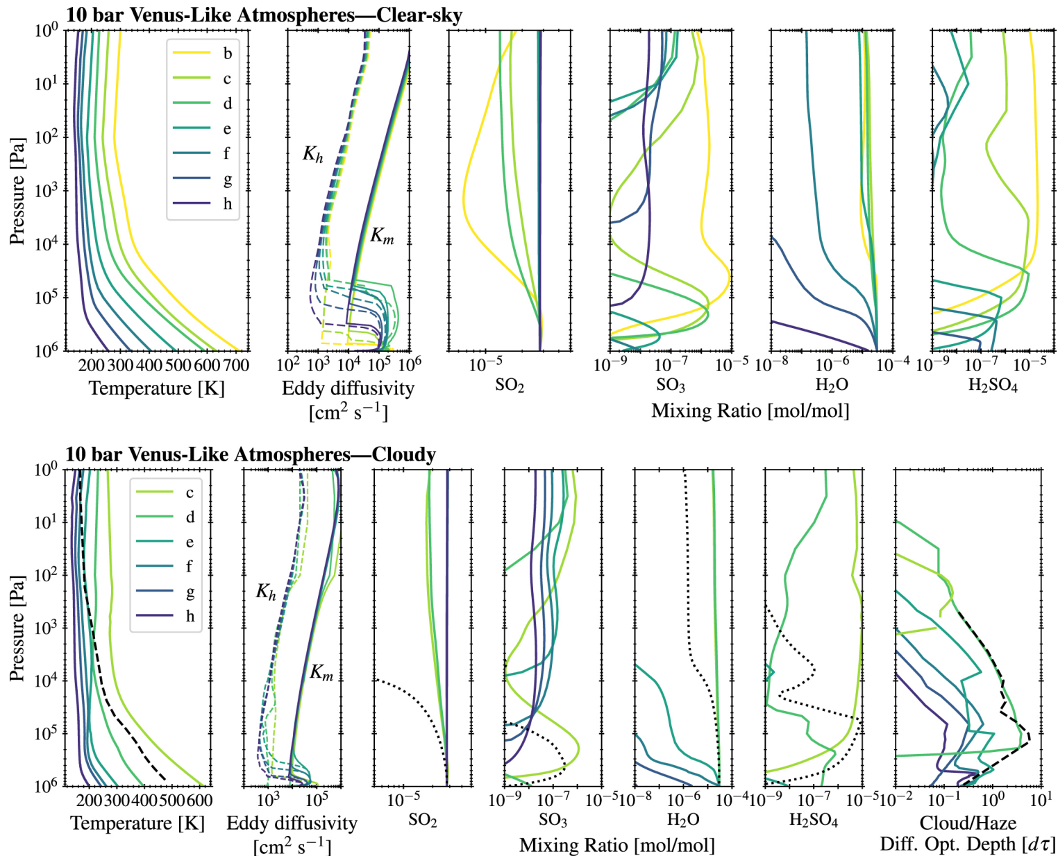
Figure 6. from Evolved Climates and Observational Discriminants for the TRAPPIST-1 Planetary System null 2018 APJ 867 76 doi:10.3847/1538-4357/aae36a https://dx.doi.org/10.3847/1538-4357/aae36a © 2018. The American Astronomical Society.
