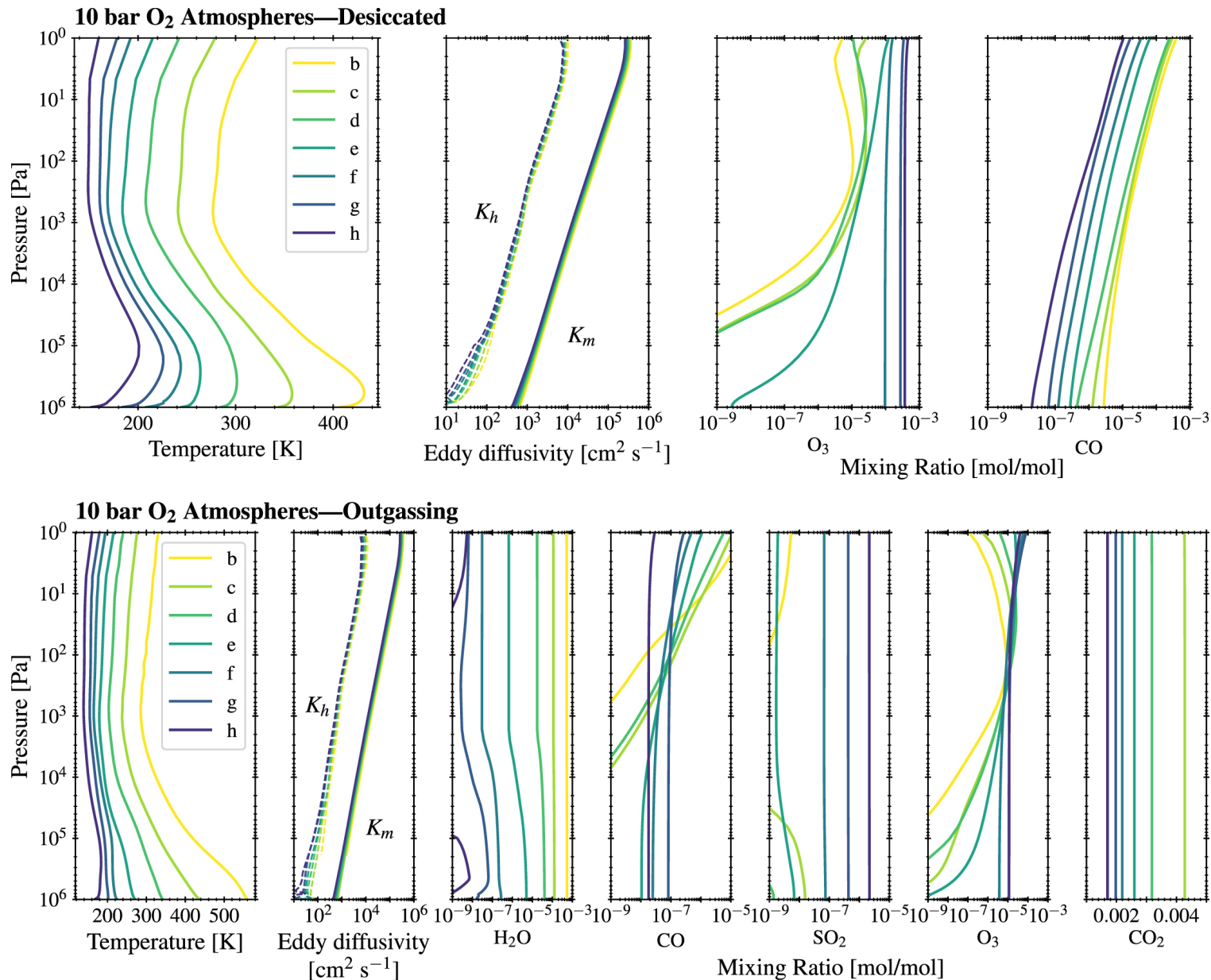
Figure 5. from Evolved Climates and Observational Discriminants for the TRAPPIST-1 Planetary System null 2018 APJ 867 76 doi:10.3847/1538-4357/aae36a https://dx.doi.org/10.3847/1538-4357/aae36a © 2018. The American Astronomical Society.
