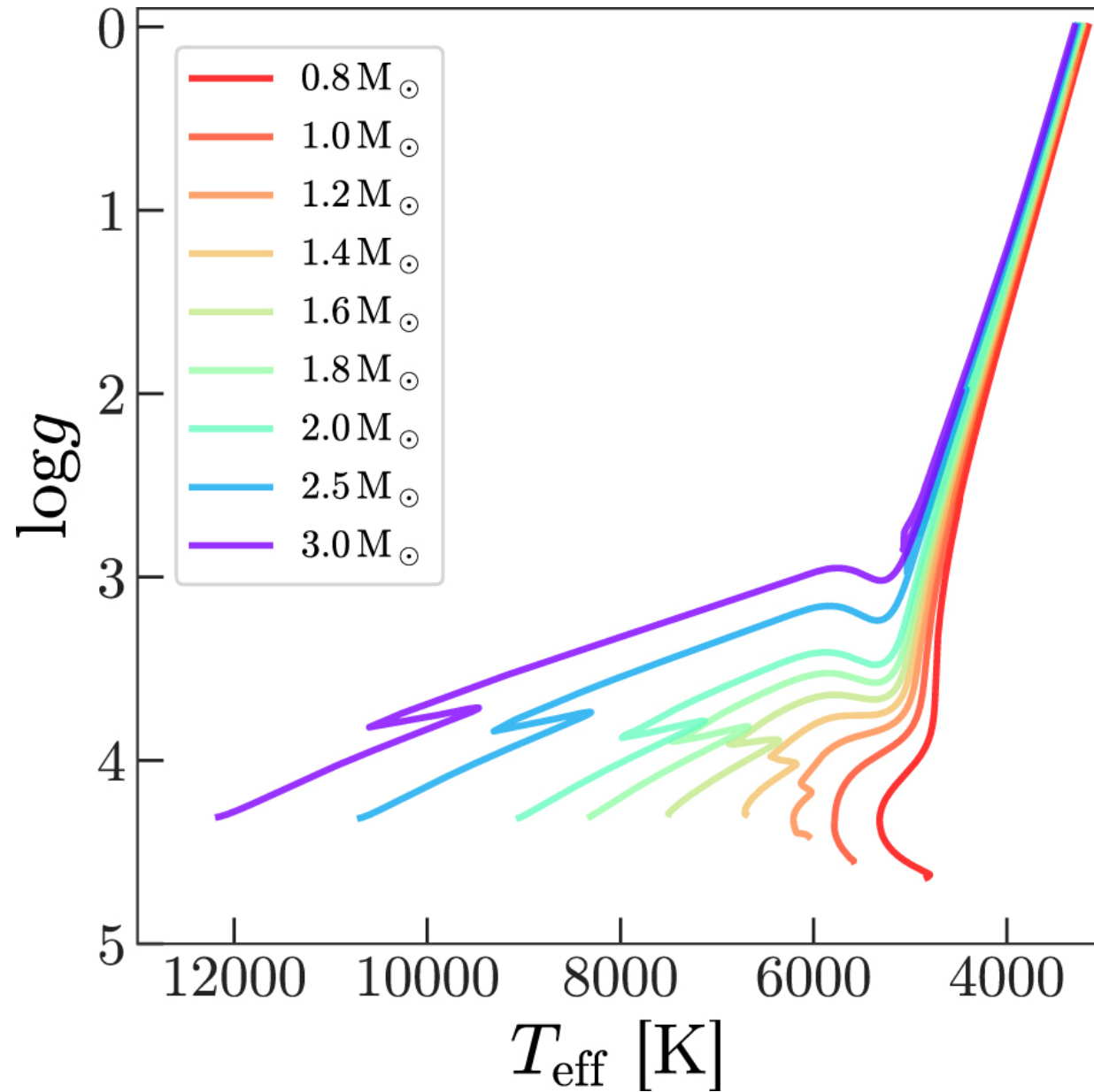
Figure 6. from Binary Companions of Evolved Stars in APOGEE DR14: Orbital Circularization null 2018 APJ 867 5 doi:10.3847/1538-4357/aae264 https://dx.doi.org/10.3847/1538-4357/aae264 © 2018. The American Astronomical Society. All rights reserved.
