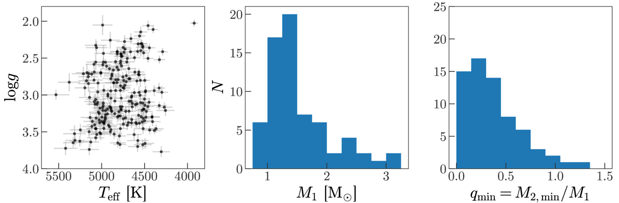
Figure 1. from Binary Companions of Evolved Stars in APOGEE DR14: Orbital Circularization null 2018 APJ 867 5 doi:10.3847/1538-4357/aae264 https://dx.doi.org/10.3847/1538-4357/aae264 © 2018. The American Astronomical Society. All rights reserved.
