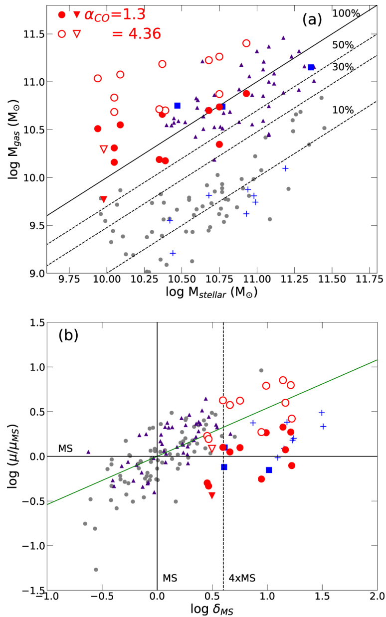
Figure 7. from The Molecular Gas Content and Fuel Efficiency of Starbursts at z \sim 1.6 with ALMA null 2018 APJ 867 92 doi:10.3847/1538-4357/aae25e https://dx.doi.org/10.3847/1538-4357/aae25e © 2018. The American Astronomical Society. All rights reserved.
