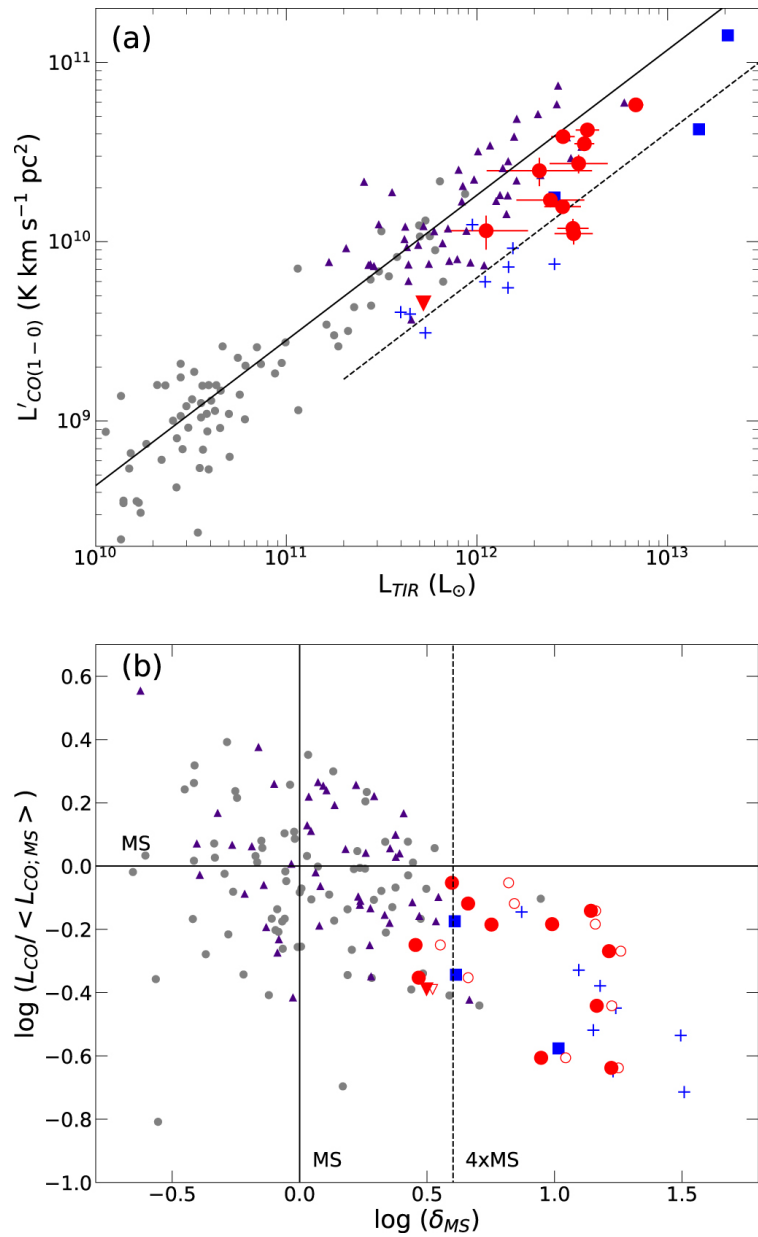
Figure 6. from The Molecular Gas Content and Fuel Efficiency of Starbursts at z \sim 1.6 with ALMA null 2018 APJ 867 92 doi:10.3847/1538-4357/aae25e https://dx.doi.org/10.3847/1538-4357/aae25e © 2018. The American Astronomical Society. All rights reserved.
