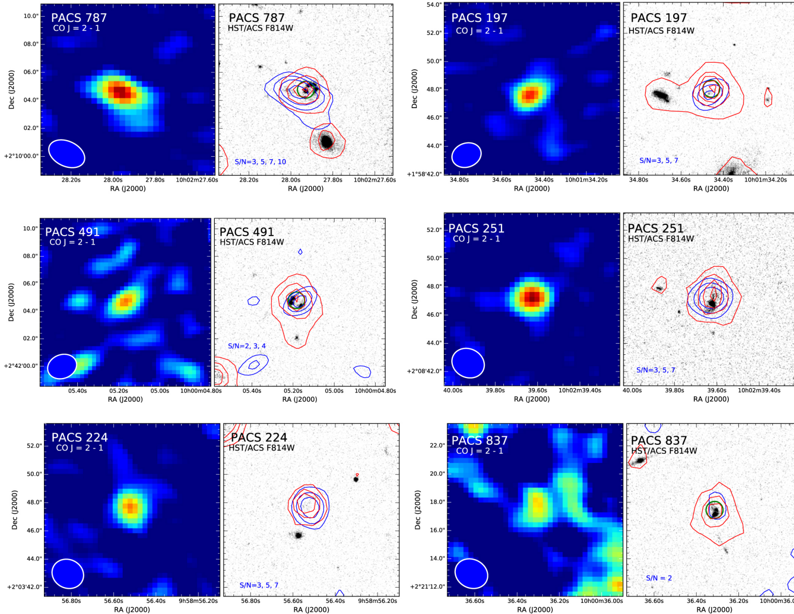
Figure 4. from The Molecular Gas Content and Fuel Efficiency of Starbursts at z \sim 1.6 with ALMA null 2018 APJ 867 92 doi:10.3847/1538-4357/aae25e https://dx.doi.org/10.3847/1538-4357/aae25e © 2018. The American Astronomical Society. All rights reserved.
