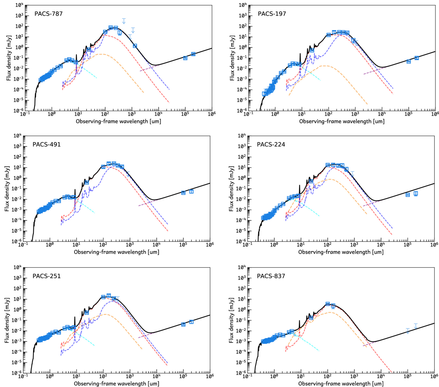
Figure 2. from The Molecular Gas Content and Fuel Efficiency of Starbursts at z \sim 1.6 with ALMA null 2018 APJ 867 92 doi:10.3847/1538-4357/aae25e https://dx.doi.org/10.3847/1538-4357/aae25e © 2018. The American Astronomical Society. All rights reserved.
