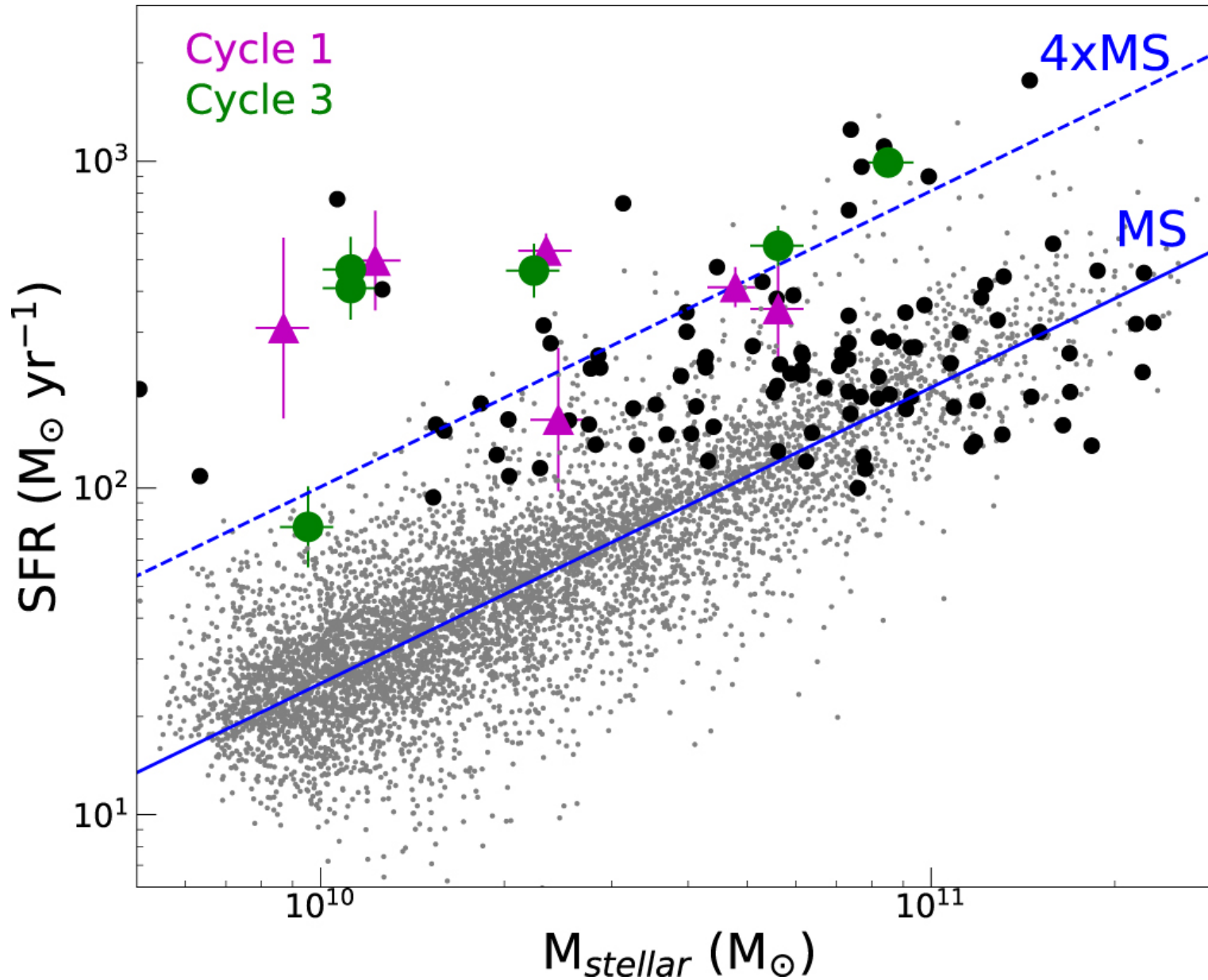
Figure 1. from The Molecular Gas Content and Fuel Efficiency of Starbursts at z \sim 1.6 with ALMA null 2018 APJ 867 92 doi:10.3847/1538-4357/aae25e https://dx.doi.org/10.3847/1538-4357/aae25e © 2018. The American Astronomical Society. All rights reserved.
