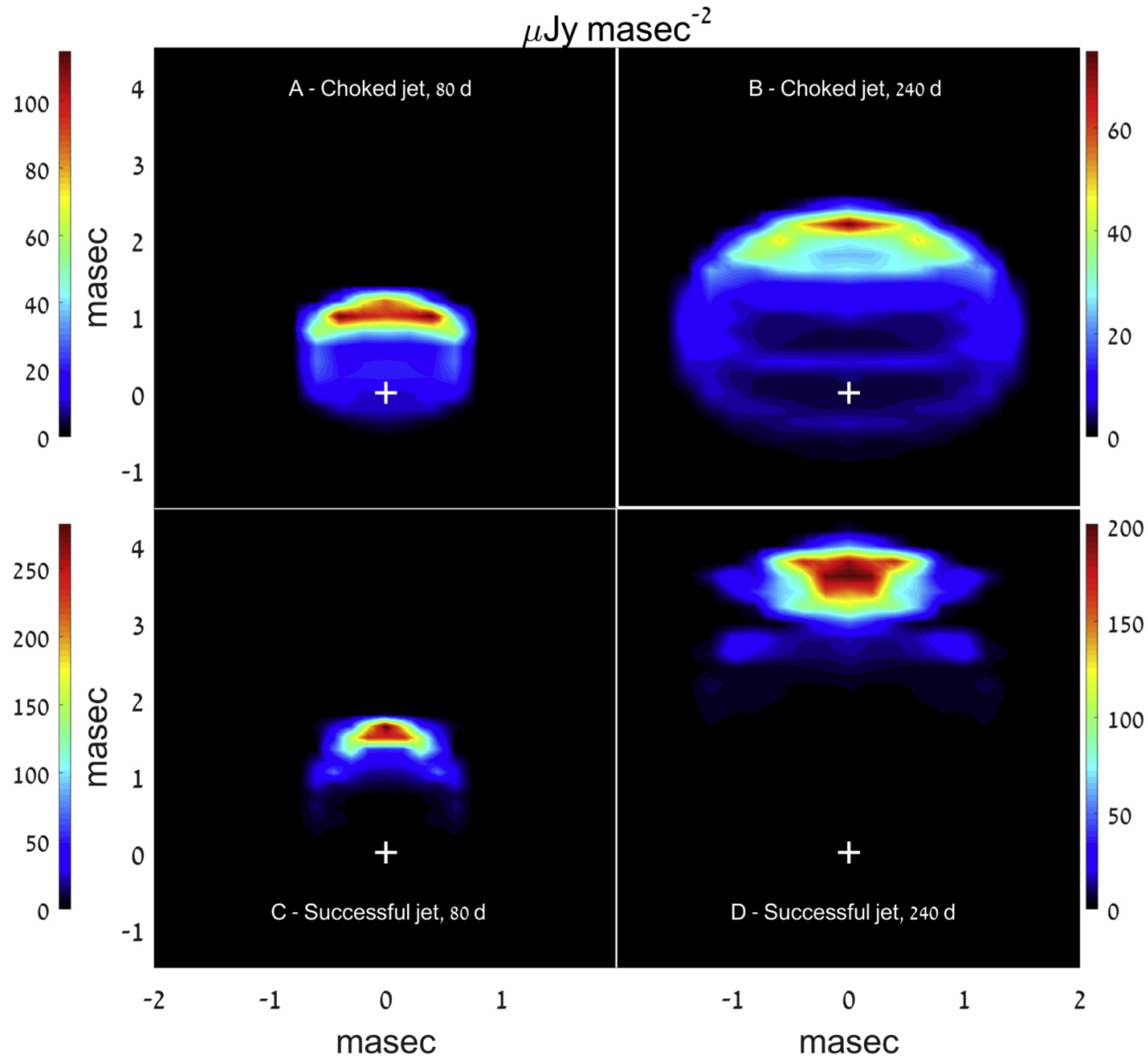
Figure 5. from From to Radio: The Electromagnetic Counterpart of GW170817 null 2018 APJ 867 18 doi:10.3847/1538-4357/aae205 https://dx.doi.org/10.3847/1538-4357/aae205 © 2018. The American Astronomical Society. All rights reserved.
