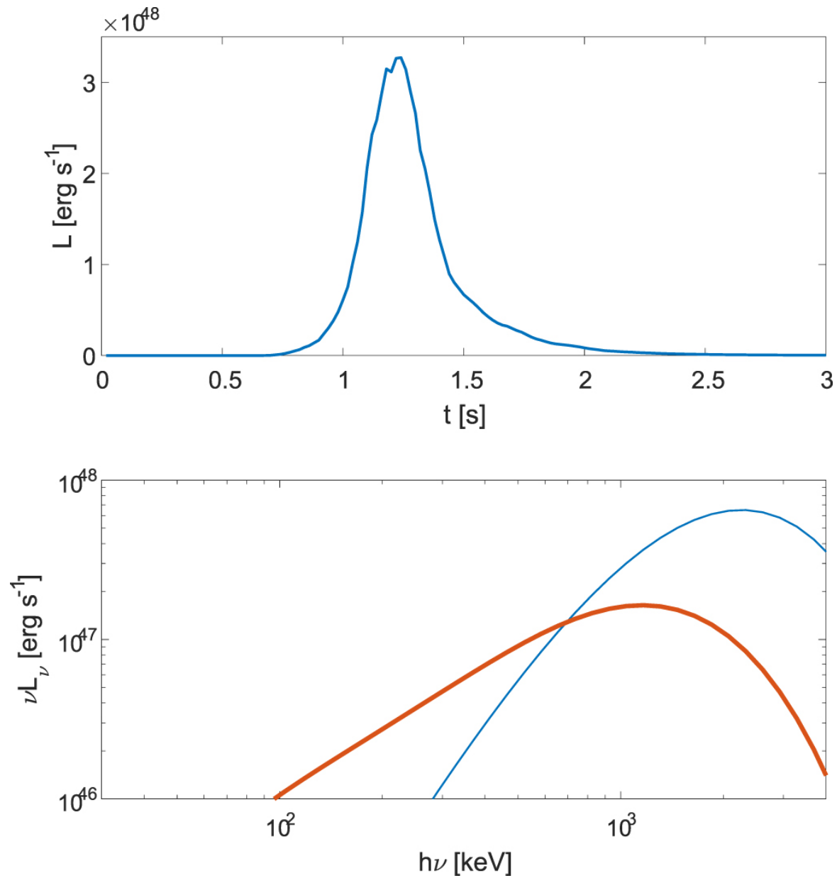
Figure 4. from From to Radio: The Electromagnetic Counterpart of GW170817 null 2018 APJ 867 18 doi:10.3847/1538-4357/aae205 https://dx.doi.org/10.3847/1538-4357/aae205 © 2018. The American Astronomical Society. All rights reserved.
