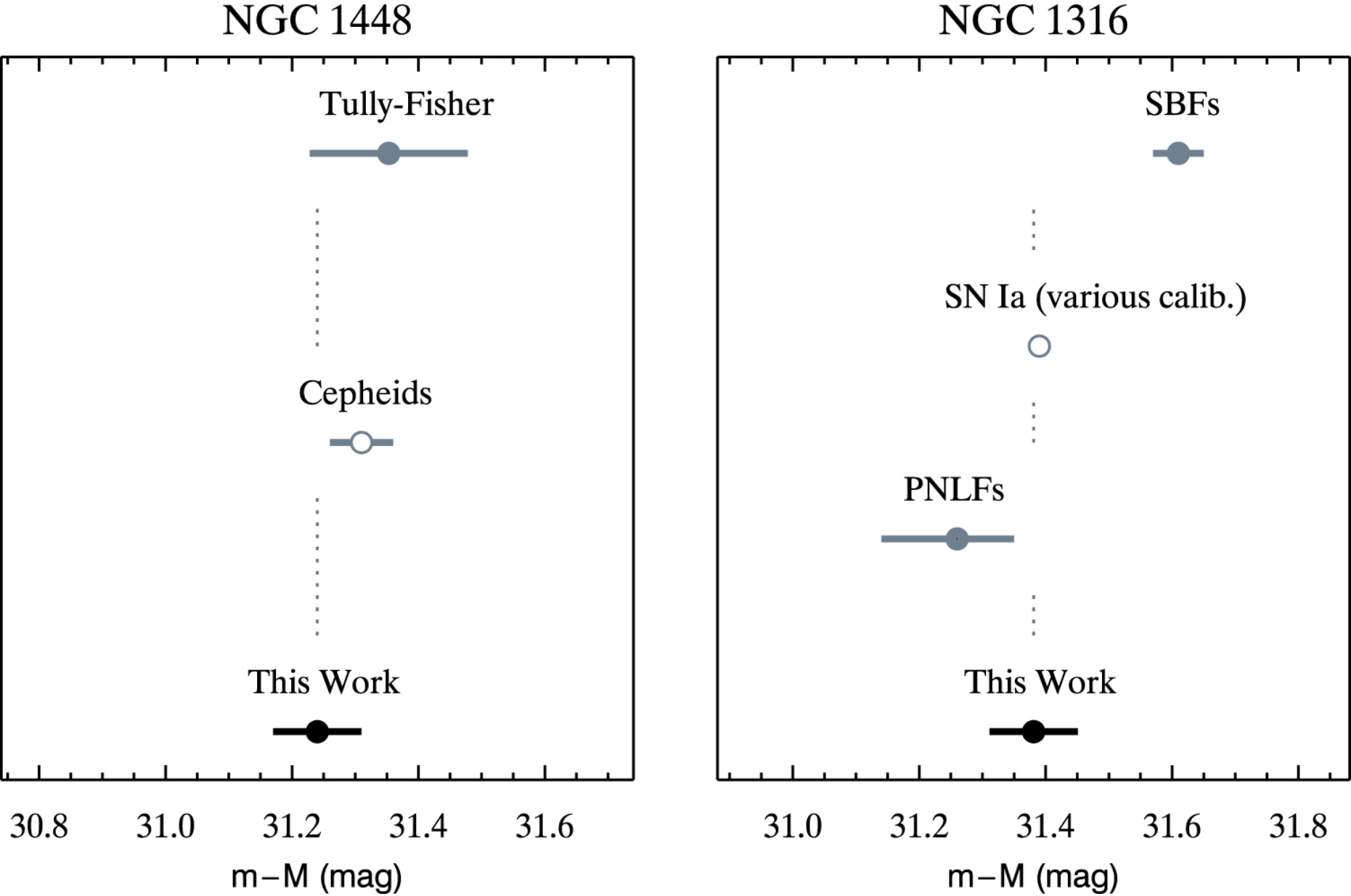
Figure 5. from The Carnegie–Chicago Hubble Program. V. The Distances to NGC 1448 and NGC 1316 via the Tip of the Red Giant Branch null 2018 APJ 866 145 doi:10.3847/1538-4357/aadfe8 https://dx.doi.org/10.3847/1538-4357/aadfe8 © 2018. The American Astronomical Society. All rights reserved.
