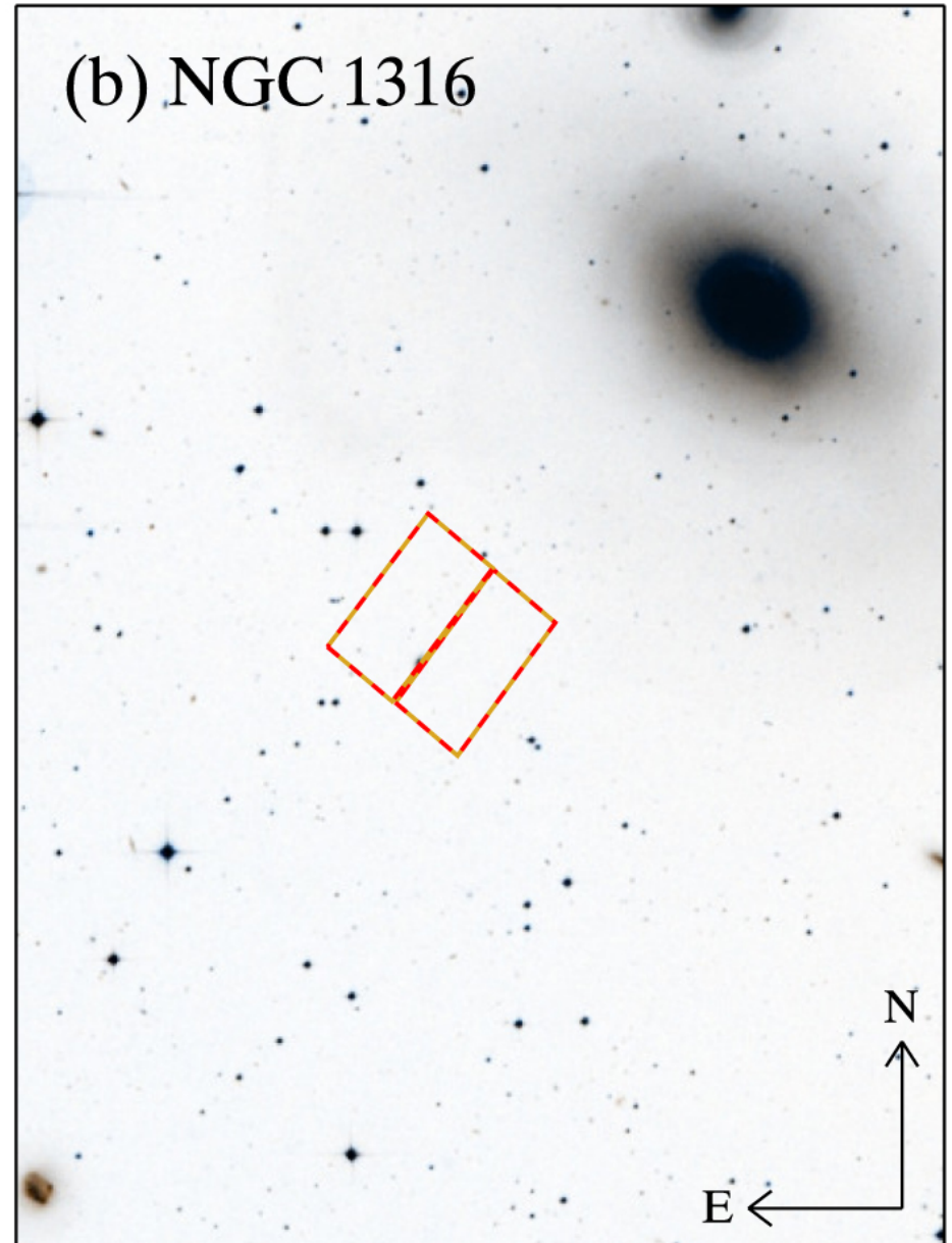
Figure 1. from The Carnegie–Chicago Hubble Program. V. The Distances to NGC 1448 and NGC 1316 via the Tip of the Red Giant Branch null 2018 APJ 866 145 doi:10.3847/1538-4357/aadfe8 https://dx.doi.org/10.3847/1538-4357/aadfe8 © 2018. The American Astronomical Society. All rights reserved.
