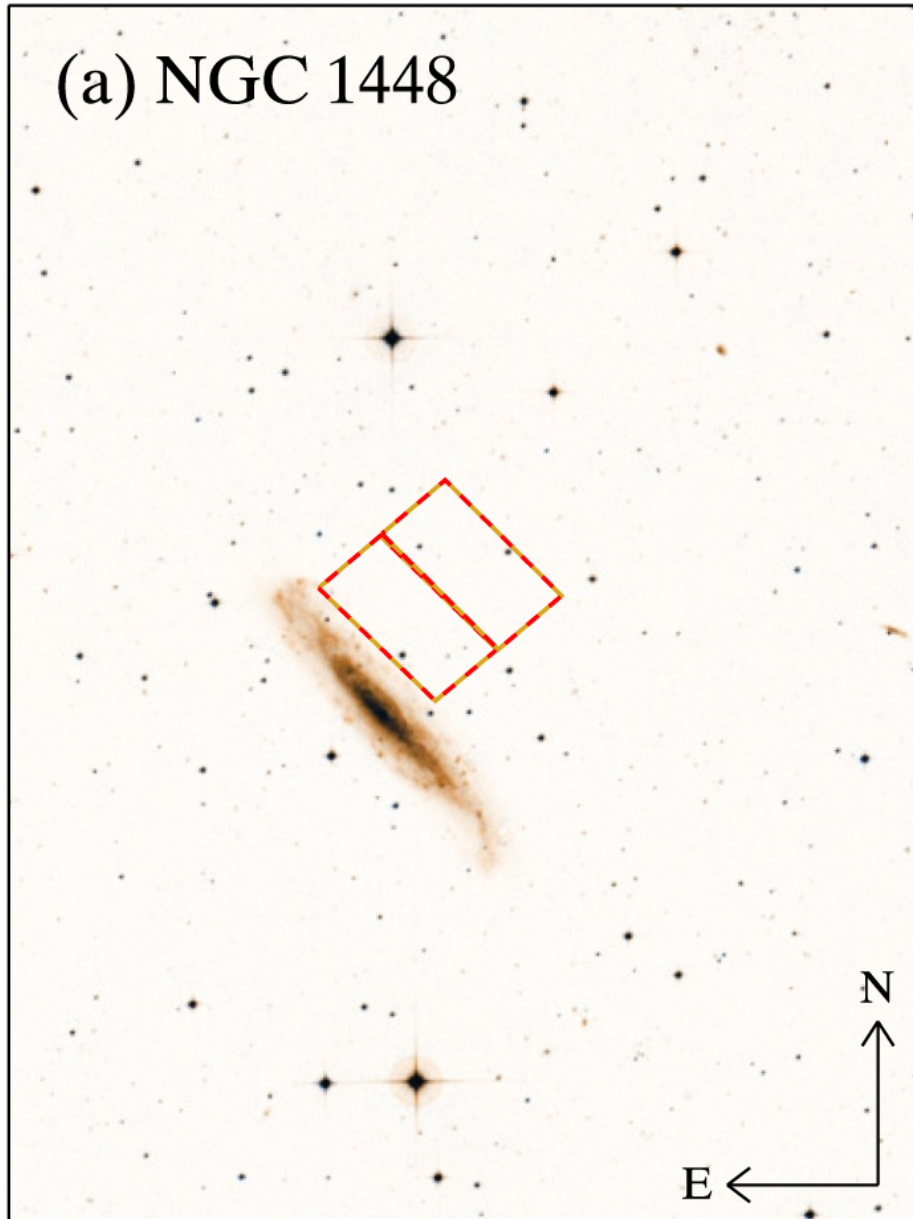
Figure 1. from The Carnegie–Chicago Hubble Program. V. The Distances to NGC 1448 and NGC 1316 via the Tip of the Red Giant Branch null 2018 APJ 866 145 doi:10.3847/1538-4357/aadfe8 https://dx.doi.org/10.3847/1538-4357/aadfe8 © 2018. The American Astronomical Society. All rights reserved.
