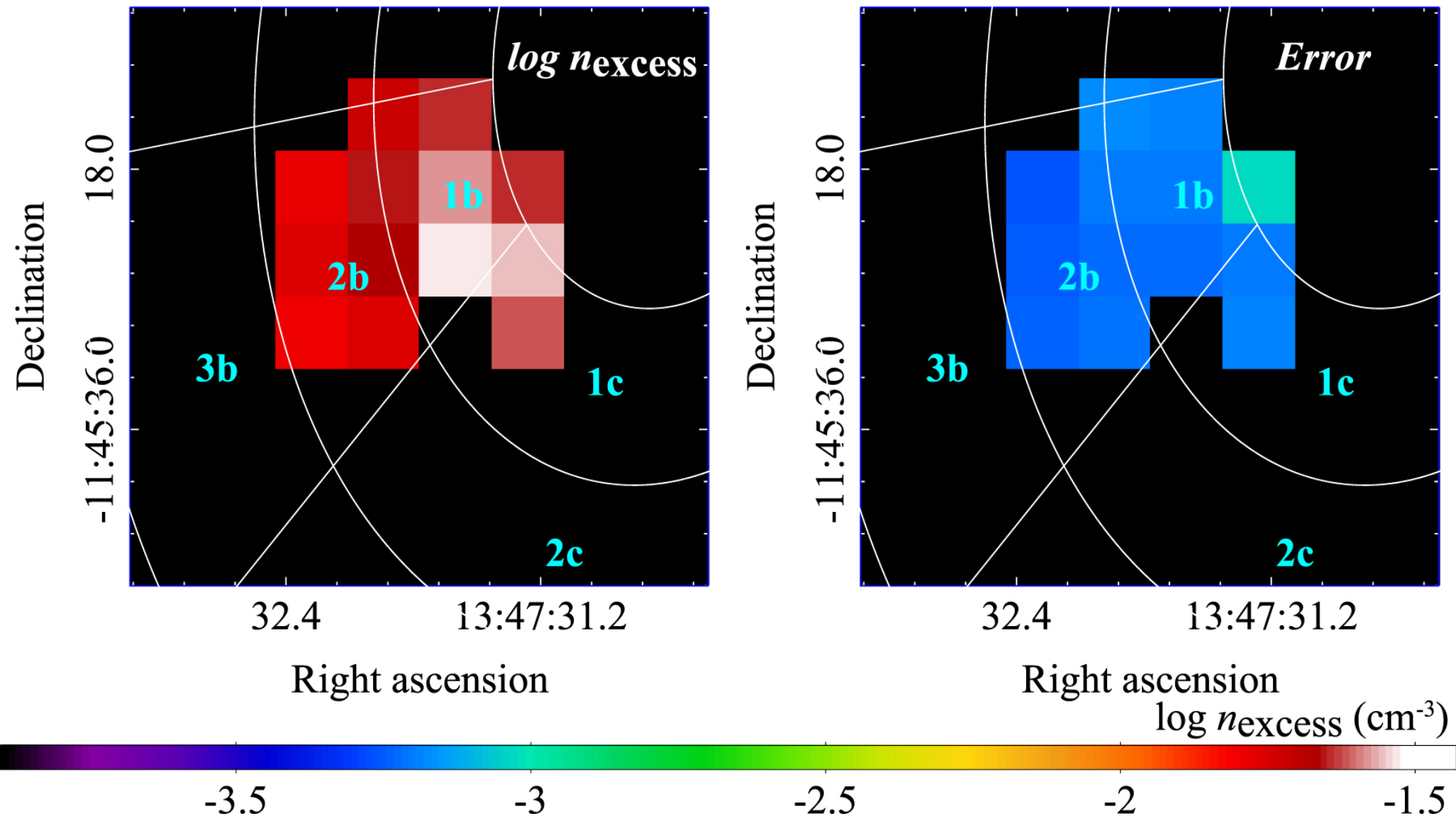
Figure 8. from A Cool Core Disturbed: Observational Evidence for the Coexistence of Subsonic Sloshing Gas and Stripped Shock-heated Gas around the Core of RX J1347.5–1145 null 2018 APJ 866 48 doi:10.3847/1538-4357/aadd9d https://dx.doi.org/10.3847/1538-4357/aadd9d © 2018. The American Astronomical Society. All rights reserved.
