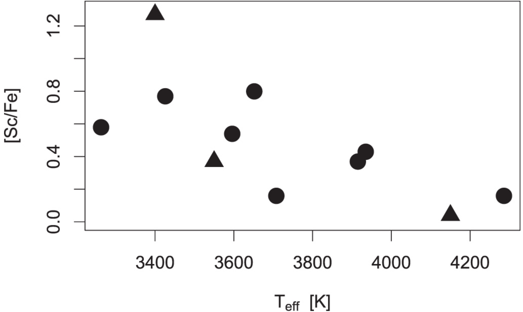
Figure 6. from Evidence against Anomalous Compositions for Giants in the Galactic Nuclear Star Cluster null 2018 APJ 866 52 doi:10.3847/1538-4357/aadb97 https://dx.doi.org/10.3847/1538-4357/aadb97 © 2018. The American Astronomical Society. All rights reserved.
