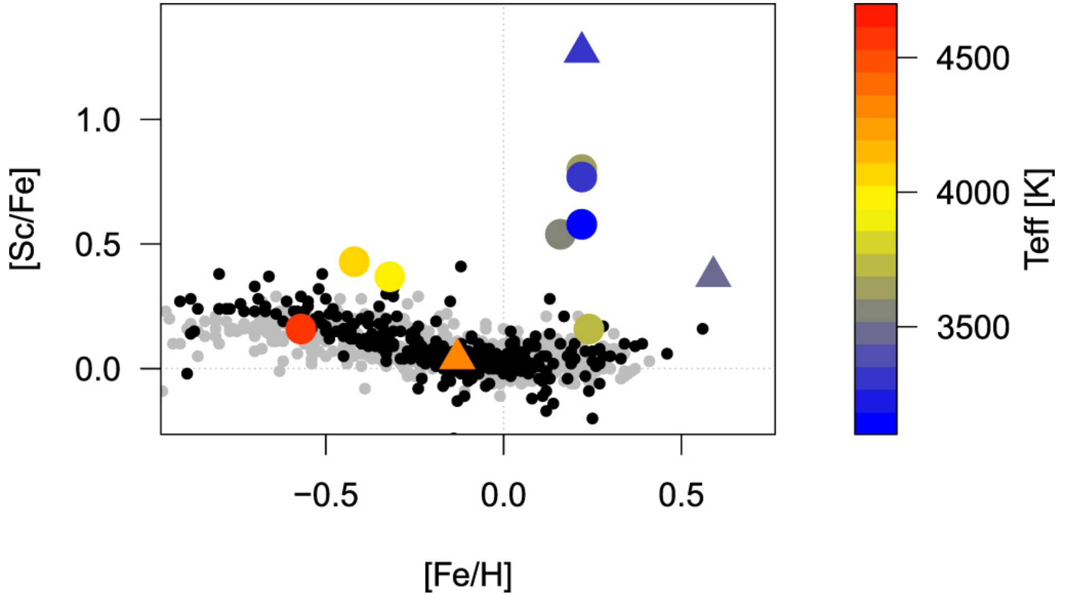
Figure 5. from Evidence against Anomalous Compositions for Giants in the Galactic Nuclear Star Cluster null 2018 APJ 866 52 doi:10.3847/1538-4357/aadb97 https://dx.doi.org/10.3847/1538-4357/aadb97 © 2018. The American Astronomical Society. All rights reserved.
