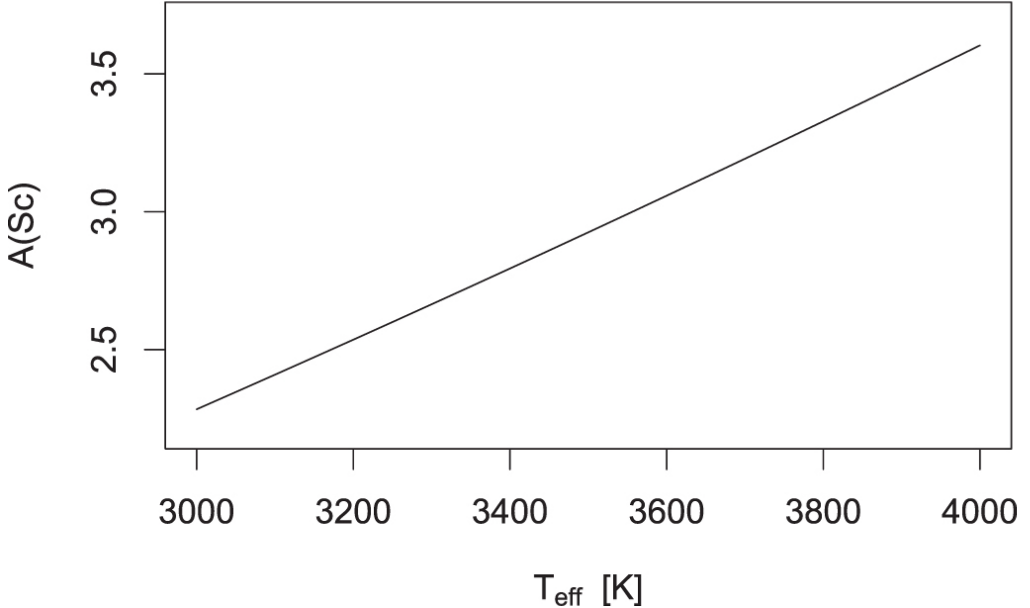
Figure 4. from Evidence against Anomalous Compositions for Giants in the Galactic Nuclear Star Cluster null 2018 APJ 866 52 doi:10.3847/1538-4357/aadb97 https://dx.doi.org/10.3847/1538-4357/aadb97 © 2018. The American Astronomical Society. All rights reserved.
