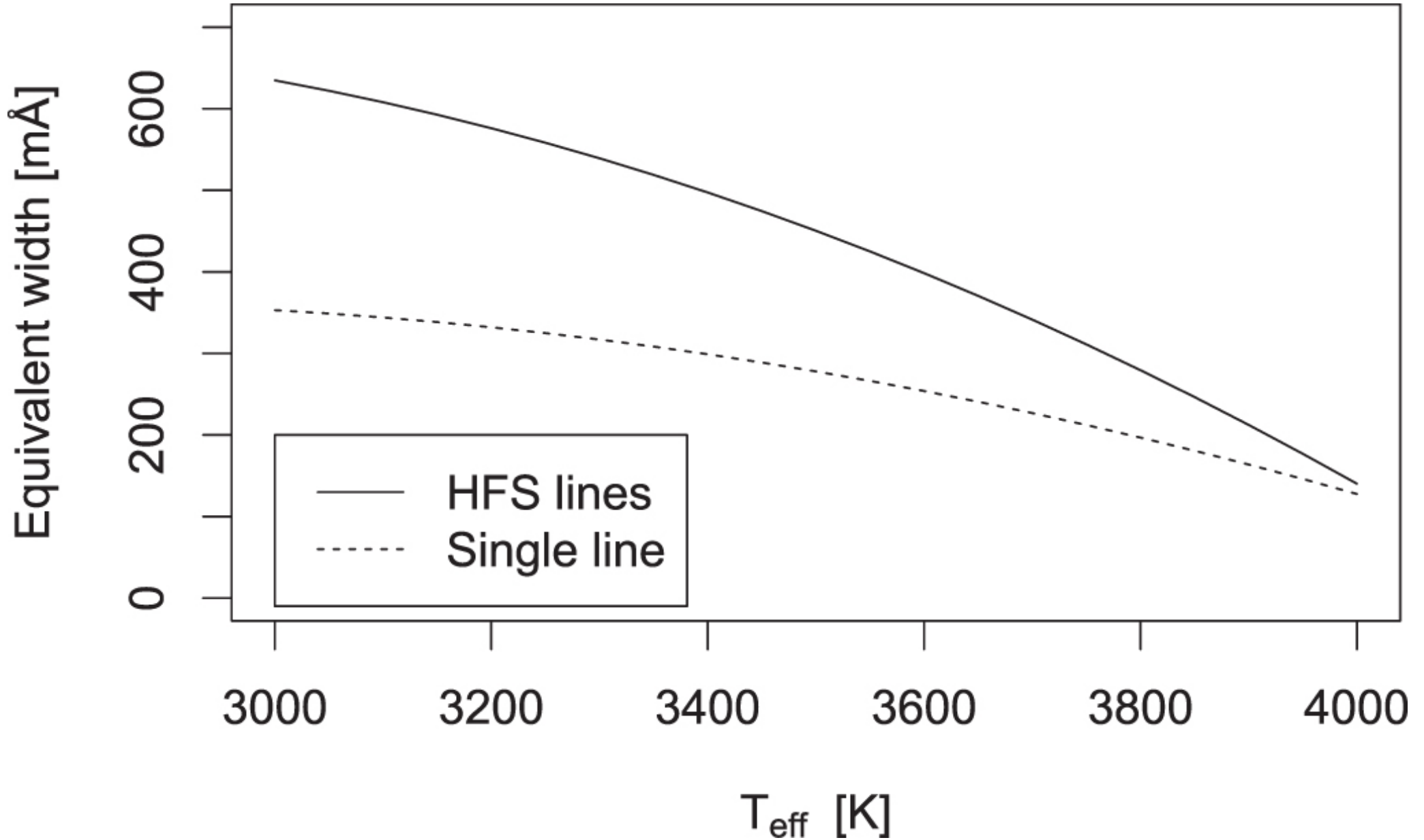
Figure 3. from Evidence against Anomalous Compositions for Giants in the Galactic Nuclear Star Cluster null 2018 APJ 866 52 doi:10.3847/1538-4357/aadb97 https://dx.doi.org/10.3847/1538-4357/aadb97 © 2018. The American Astronomical Society. All rights reserved.
