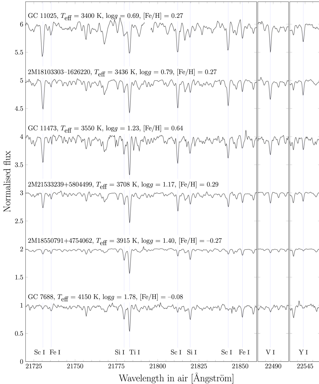
Figure 1. from Evidence against Anomalous Compositions for Giants in the Galactic Nuclear Star Cluster null 2018 APJ 866 52 doi:10.3847/1538-4357/aadb97 https://dx.doi.org/10.3847/1538-4357/aadb97 © 2018. The American Astronomical Society. All rights reserved.
