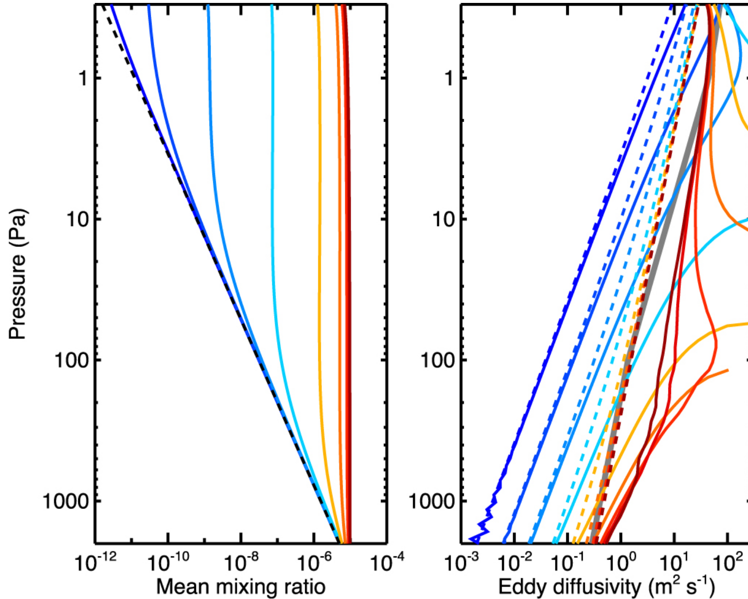
Figure 6. from Global-mean Vertical Tracer Mixing in Planetary Atmospheres. I. Theory and Fast-rotating Planets null 2018 APJ 866 1 doi:10.3847/1538-4357/aada85 https://dx.doi.org/10.3847/1538-4357/aada85 © 2018. The American Astronomical Society. All rights reserved.
