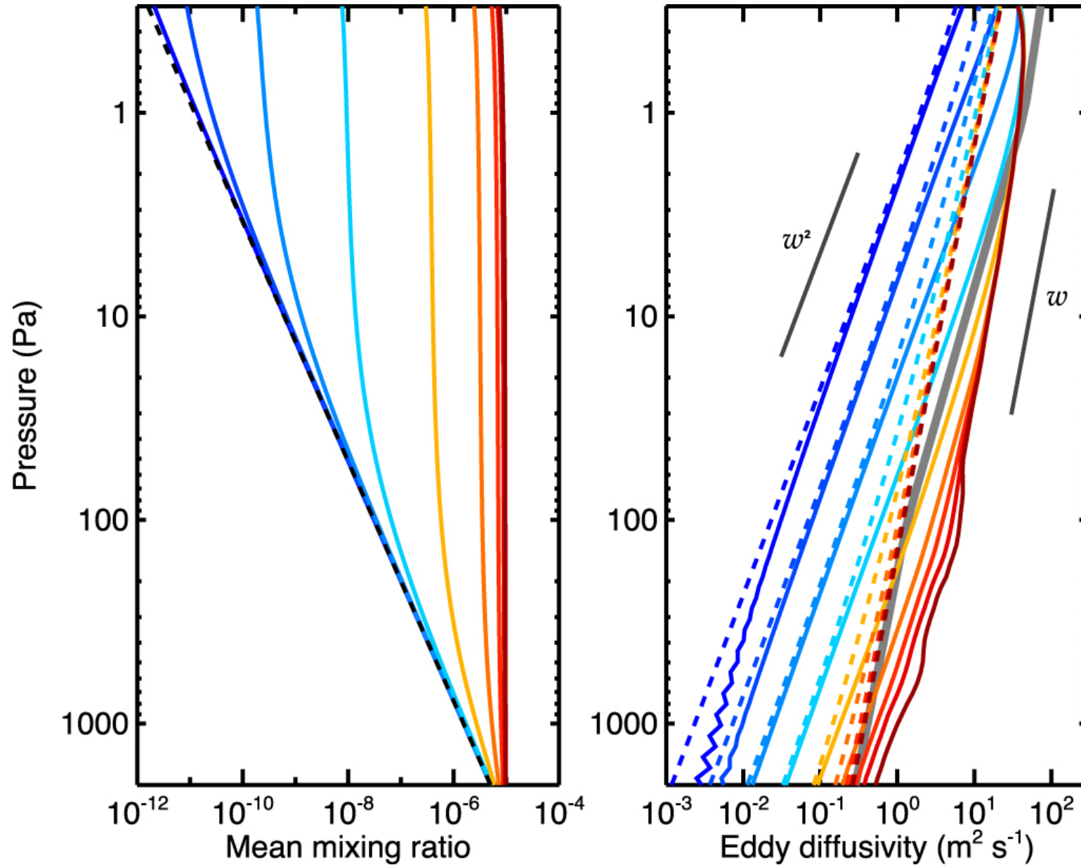
Figure 5. from Global-mean Vertical Tracer Mixing in Planetary Atmospheres. I. Theory and Fast-rotating Planets null 2018 APJ 866 1 doi:10.3847/1538-4357/aada85 https://dx.doi.org/10.3847/1538-4357/aada85 © 2018. The American Astronomical Society. All rights reserved.
