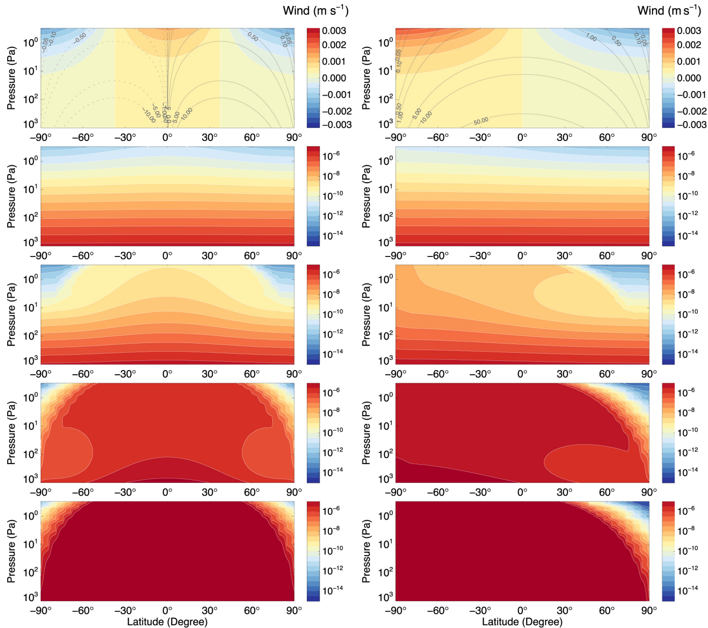
Figure 4. from Global-mean Vertical Tracer Mixing in Planetary Atmospheres. I. Theory and Fast-rotating Planets null 2018 APJ 866 1 doi:10.3847/1538-4357/aada85 https://dx.doi.org/10.3847/1538-4357/aada85 © 2018. The American Astronomical Society. All rights reserved.
