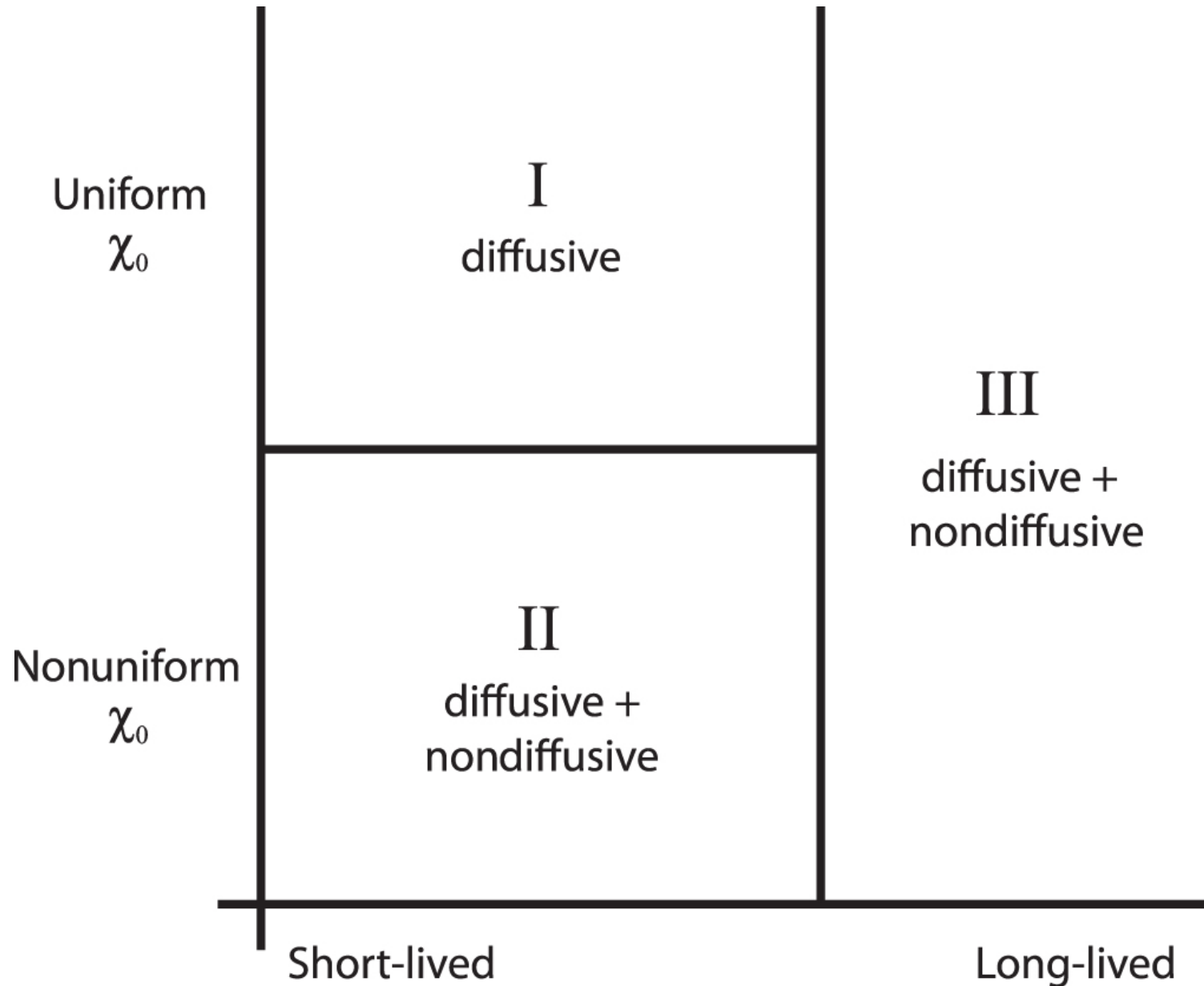
Figure 3. from Global-mean Vertical Tracer Mixing in Planetary Atmospheres. I. Theory and Fast-rotating Planets null 2018 APJ 866 1 doi:10.3847/1538-4357/aada85 https://dx.doi.org/10.3847/1538-4357/aada85 © 2018. The American Astronomical Society. All rights reserved.
