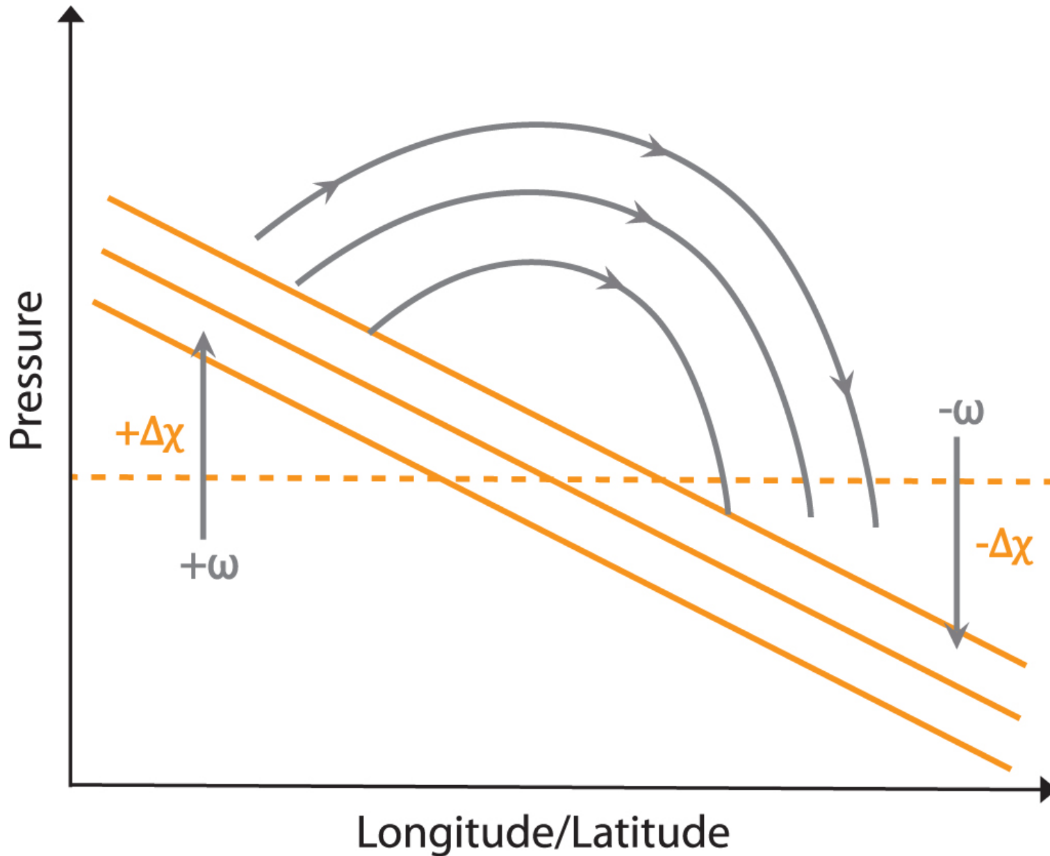
Figure 2. from Global-mean Vertical Tracer Mixing in Planetary Atmospheres. I. Theory and Fast-rotating Planets null 2018 APJ 866 1 doi:10.3847/1538-4357/aada85 https://dx.doi.org/10.3847/1538-4357/aada85 © 2018. The American Astronomical Society. All rights reserved.
