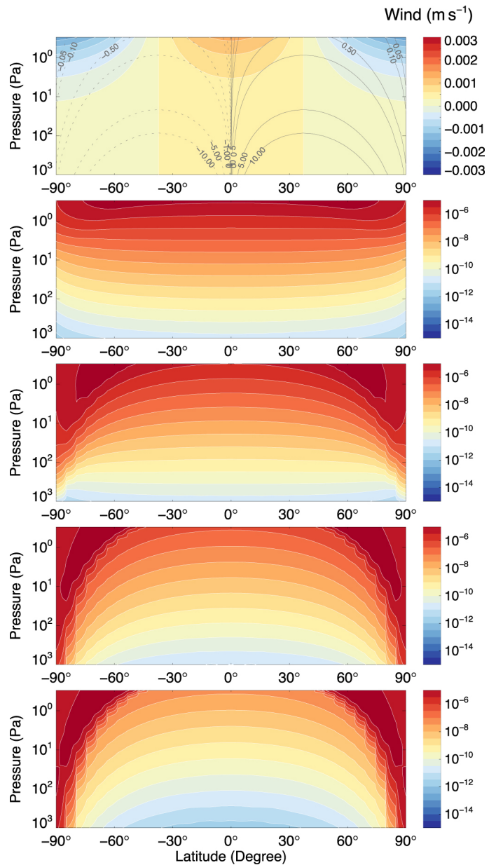
Figure 10. from Global-mean Vertical Tracer Mixing in Planetary Atmospheres. I. Theory and Fast-rotating Planets null 2018 APJ 866 1 doi:10.3847/1538-4357/aada85 https://dx.doi.org/10.3847/1538-4357/aada85 © 2018. The American Astronomical Society. All rights reserved.
