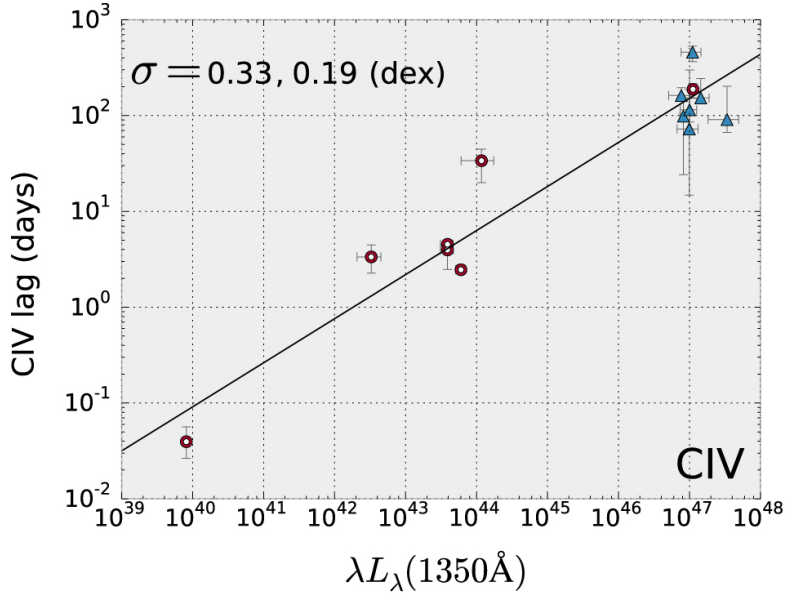
Figure 7. from Reverberation Mapping of Luminous Quasars at High z null 2018 APJ 865 56 doi:10.3847/1538-4357/aada45 https://dx.doi.org/10.3847/1538-4357/aada45 © 2018. The American Astronomical Society. All rights reserved.
