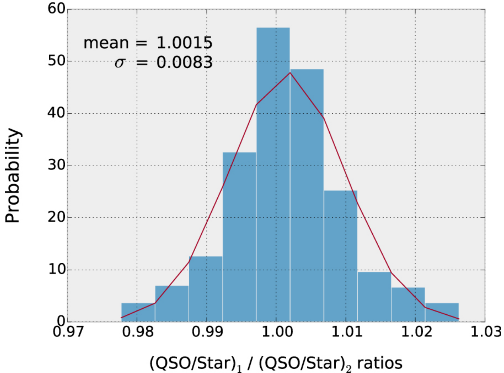
Figure 4. from Reverberation Mapping of Luminous Quasars at High z null 2018 APJ 865 56 doi:10.3847/1538-4357/aada45 https://dx.doi.org/10.3847/1538-4357/aada45 © 2018. The American Astronomical Society. All rights reserved.
