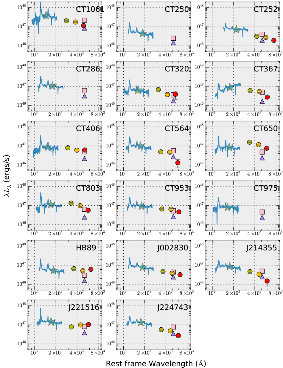
Figure 2. from Reverberation Mapping of Luminous Quasars at High z null 2018 APJ 865 56 doi:10.3847/1538-4357/aada45 https://dx.doi.org/10.3847/1538-4357/aada45
