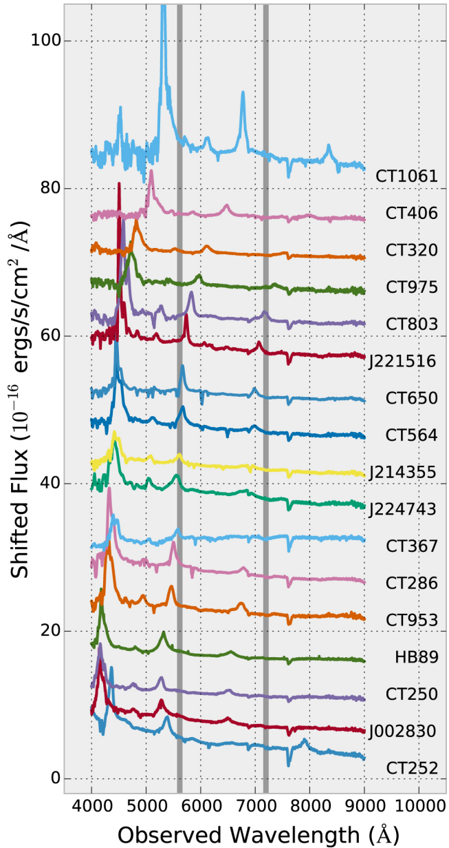
Figure 1. from Reverberation Mapping of Luminous Quasars at High z null 2018 APJ 865 56 doi:10.3847/1538-4357/aada45 https://dx.doi.org/10.3847/1538-4357/aada45 © 2018. The American Astronomical Society. All rights reserved.
