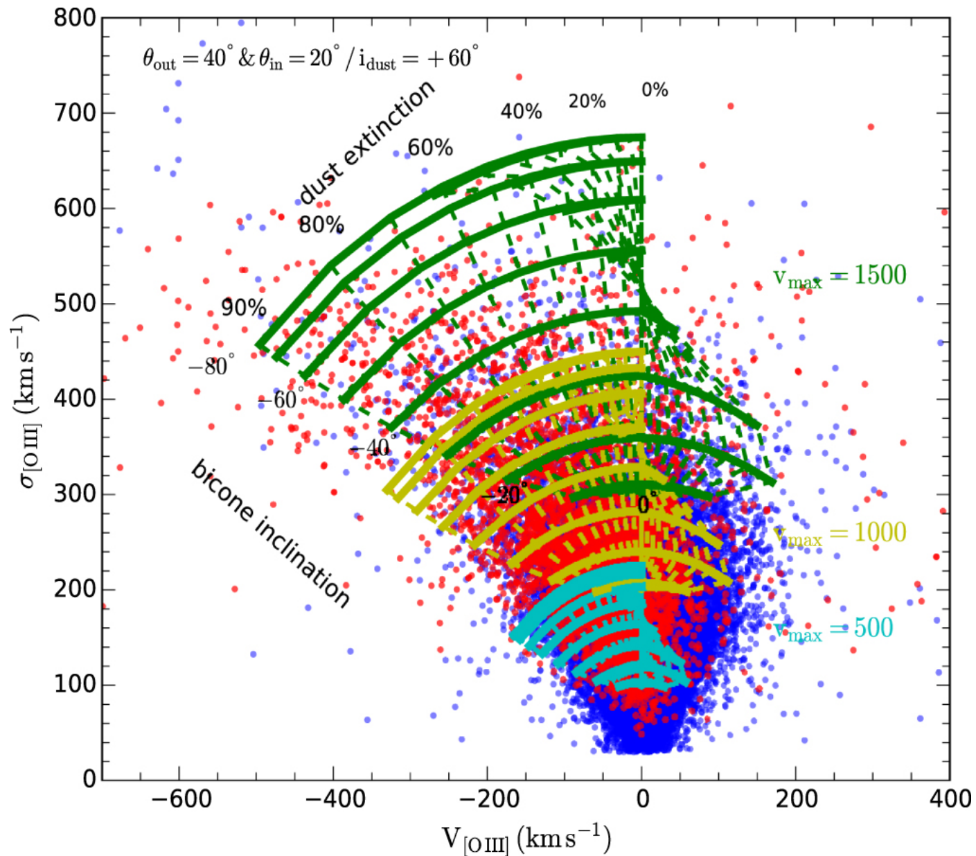
Figure 9. from A Census of Ionized Gas Outflows in Type 1 AGNs: Gas Outflows in AGNs. V. null 2018 APJ 865 5 doi:10.3847/1538-4357/aad9f8 https://dx.doi.org/10.3847/1538-4357/aad9f8 © 2018. The American Astronomical Society. All rights reserved.
