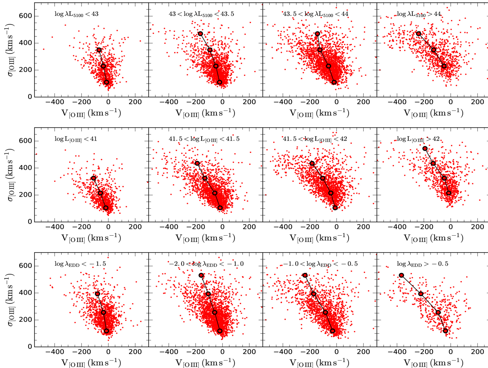
Figure 8. from A Census of Ionized Gas Outflows in Type 1 AGNs: Gas Outflows in AGNs. V. null 2018 APJ 865 5 doi:10.3847/1538-4357/aad9f8 https://dx.doi.org/10.3847/1538-4357/aad9f8 © 2018. The American Astronomical Society. All rights reserved.
