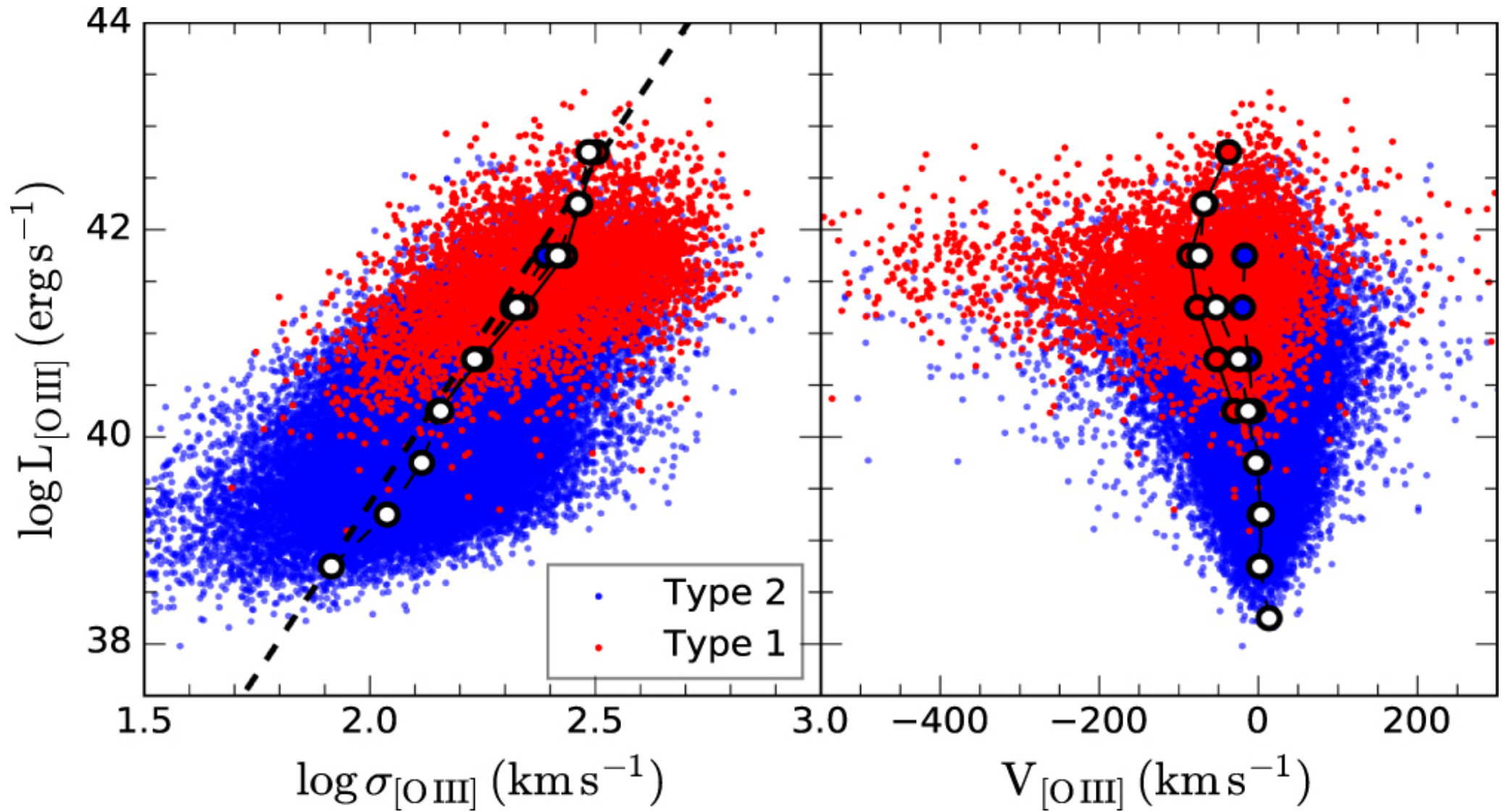
Figure 6. from A Census of Ionized Gas Outflows in Type 1 AGNs: Gas Outflows in AGNs. V. null 2018 APJ 865 5 doi:10.3847/1538-4357/aad9f8 https://dx.doi.org/10.3847/1538-4357/aad9f8 © 2018. The American Astronomical Society. All rights reserved.
