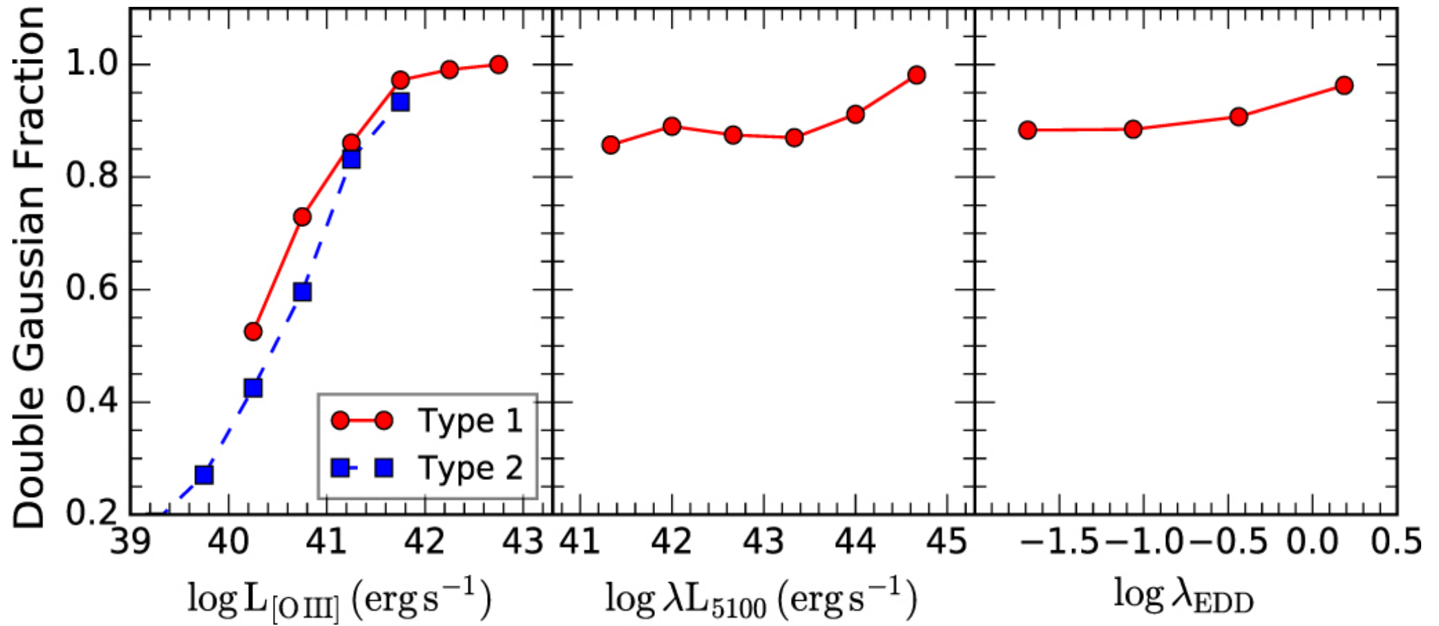
Figure 5. from A Census of Ionized Gas Outflows in Type 1 AGNs: Gas Outflows in AGNs. V. null 2018 APJ 865 5 doi:10.3847/1538-4357/aad9f8 https://dx.doi.org/10.3847/1538-4357/aad9f8 © 2018. The American Astronomical Society. All rights reserved.
