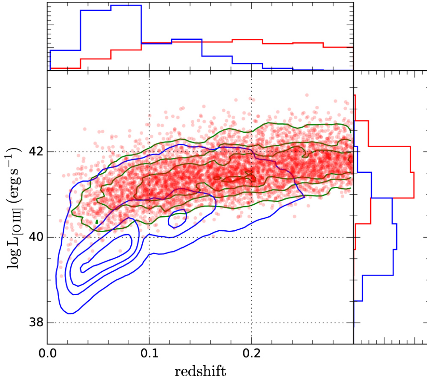
Figure 3. from A Census of Ionized Gas Outflows in Type 1 AGNs: Gas Outflows in AGNs. V. null 2018 APJ 865 5 doi:10.3847/1538-4357/aad9f8 https://dx.doi.org/10.3847/1538-4357/aad9f8 © 2018. The American Astronomical Society. All rights reserved.
