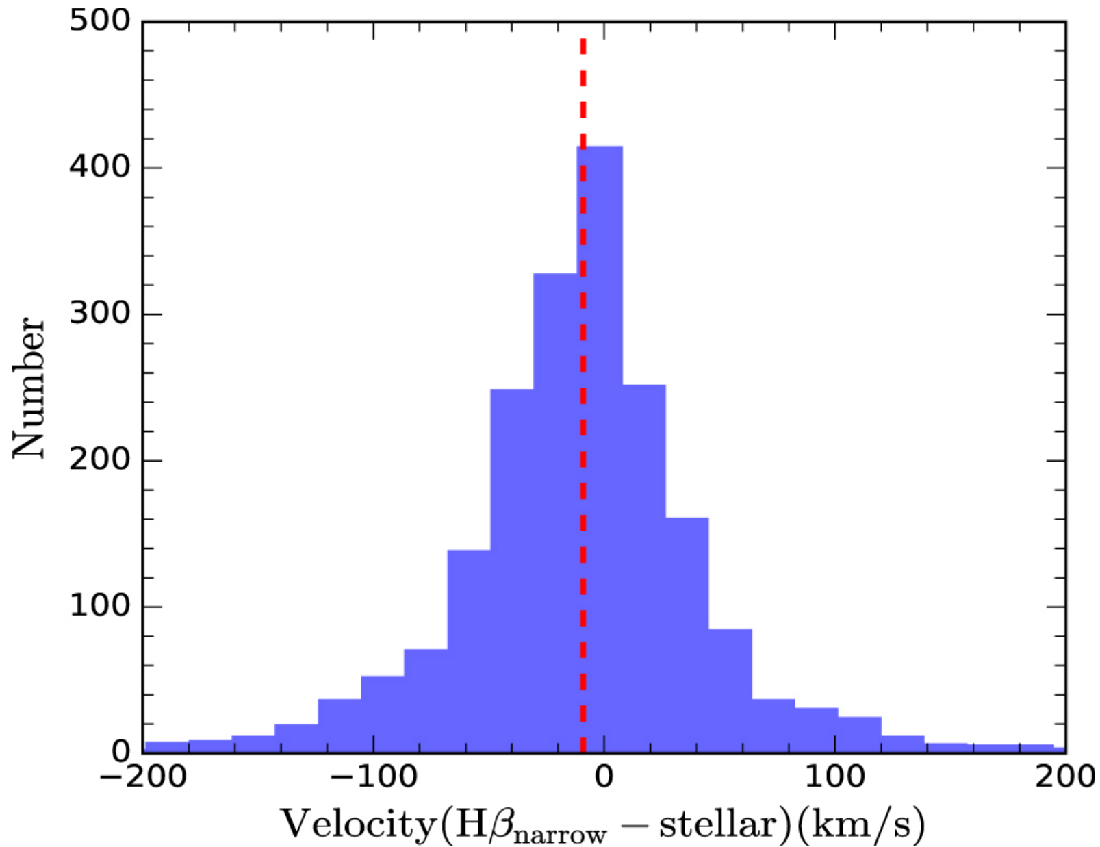
Figure 2. from A Census of Ionized Gas Outflows in Type 1 AGNs: Gas Outflows in AGNs. V. null 2018 APJ 865 5 doi:10.3847/1538-4357/aad9f8 https://dx.doi.org/10.3847/1538-4357/aad9f8 © 2018. The American Astronomical Society. All rights reserved.
