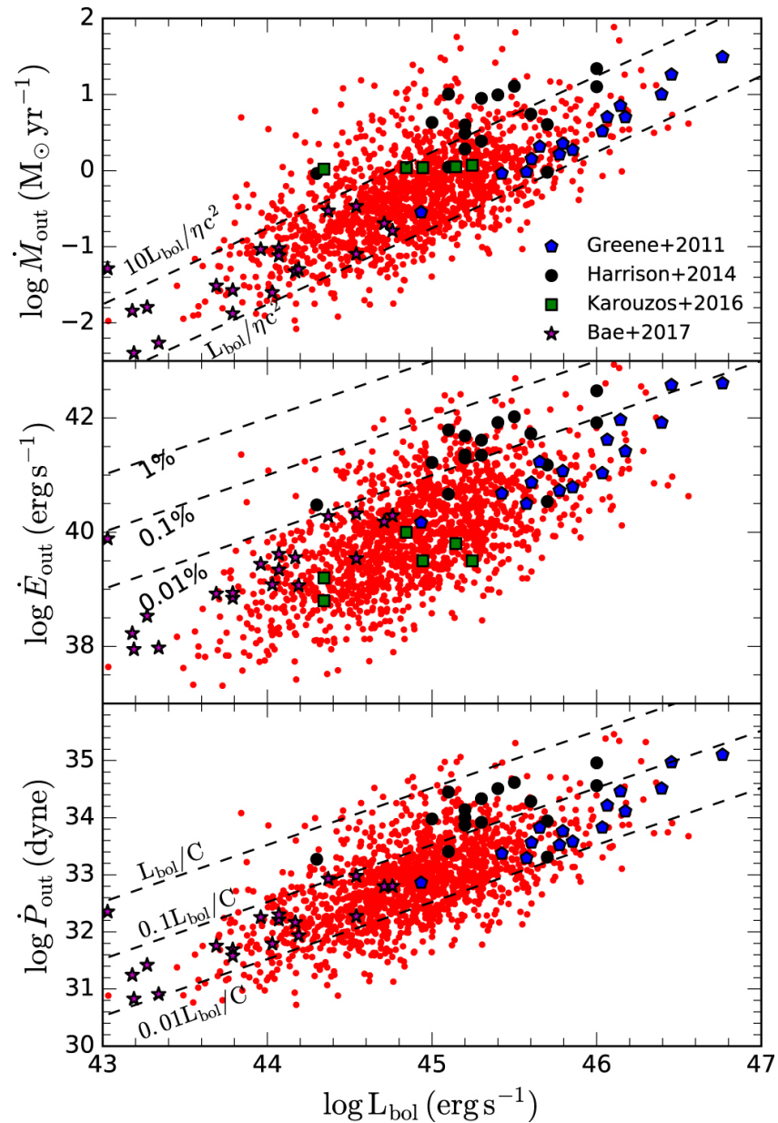
Figure 11. from A Census of Ionized Gas Outflows in Type 1 AGNs: Gas Outflows in AGNs. V. null 2018 APJ 865 5 doi:10.3847/1538-4357/aad9f8 https://dx.doi.org/10.3847/1538-4357/aad9f8 © 2018. The American Astronomical Society. All rights reserved.
