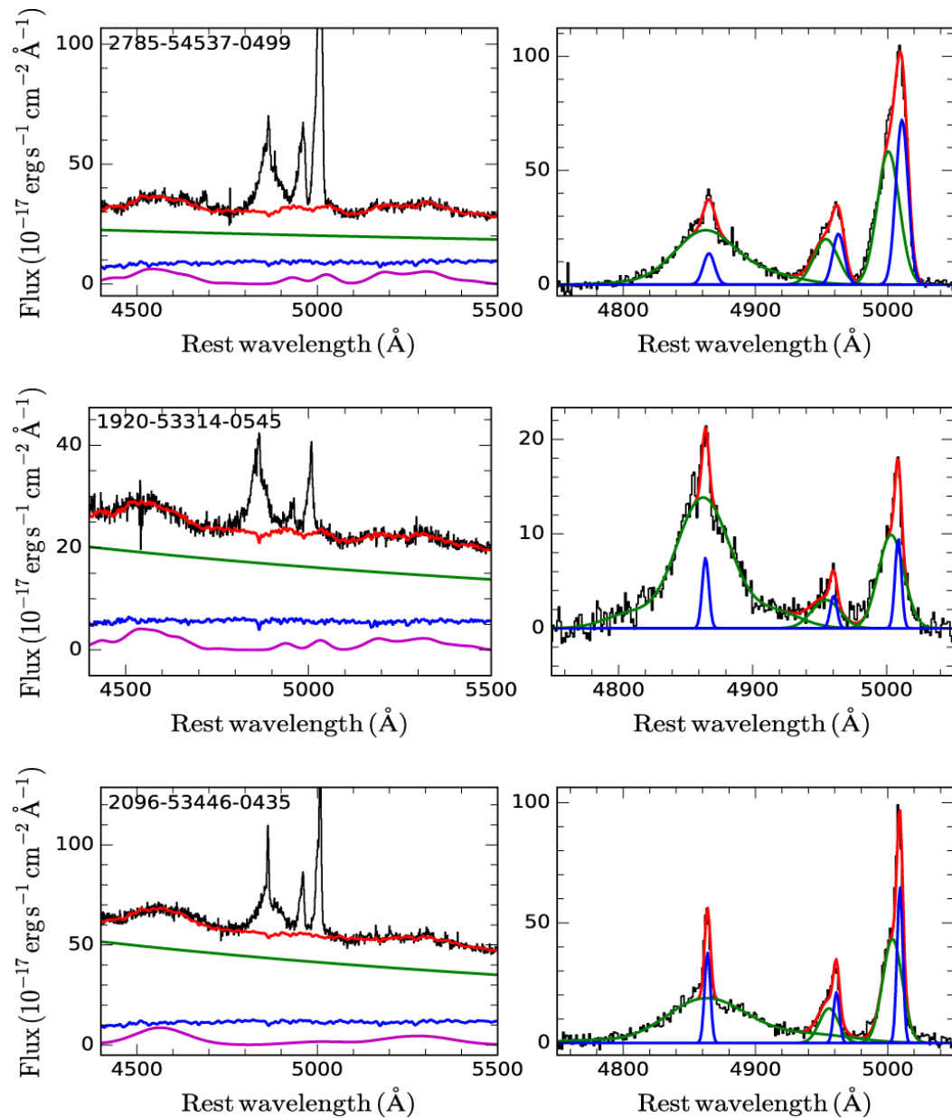
Figure 1. from A Census of Ionized Gas Outflows in Type 1 AGNs: Gas Outflows in AGNs. V. null 2018 APJ 865 5 doi:10.3847/1538-4357/aad9f8 https://dx.doi.org/10.3847/1538-4357/aad9f8 © 2018. The American Astronomical Society. All rights reserved.
