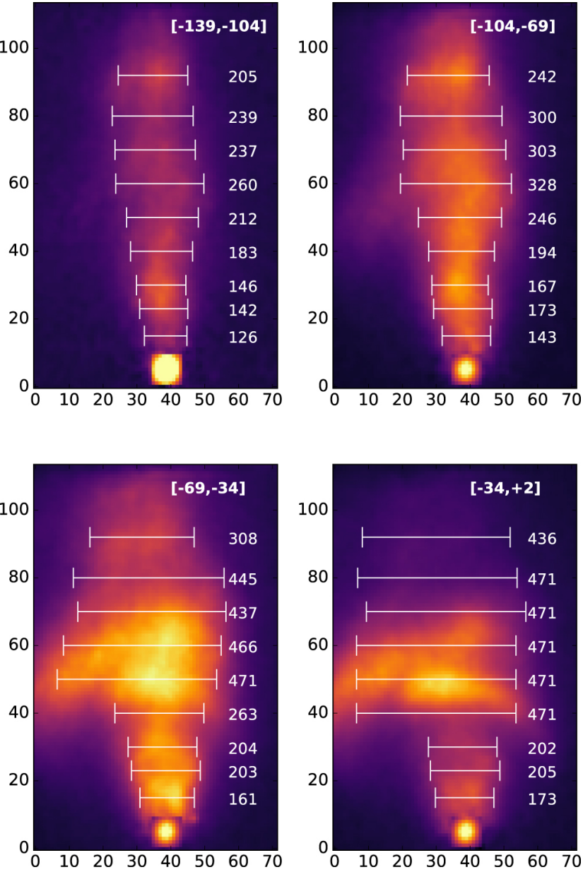
Figure 8. from Variability and Jet Activity in the YSO MHO 3252 Y3 in Serpens South null 2018 APJ 864 172 doi:10.3847/1538-4357/aad636 https://dx.doi.org/10.3847/1538-4357/aad636 © 2018. The American Astronomical Society. All rights reserved.
