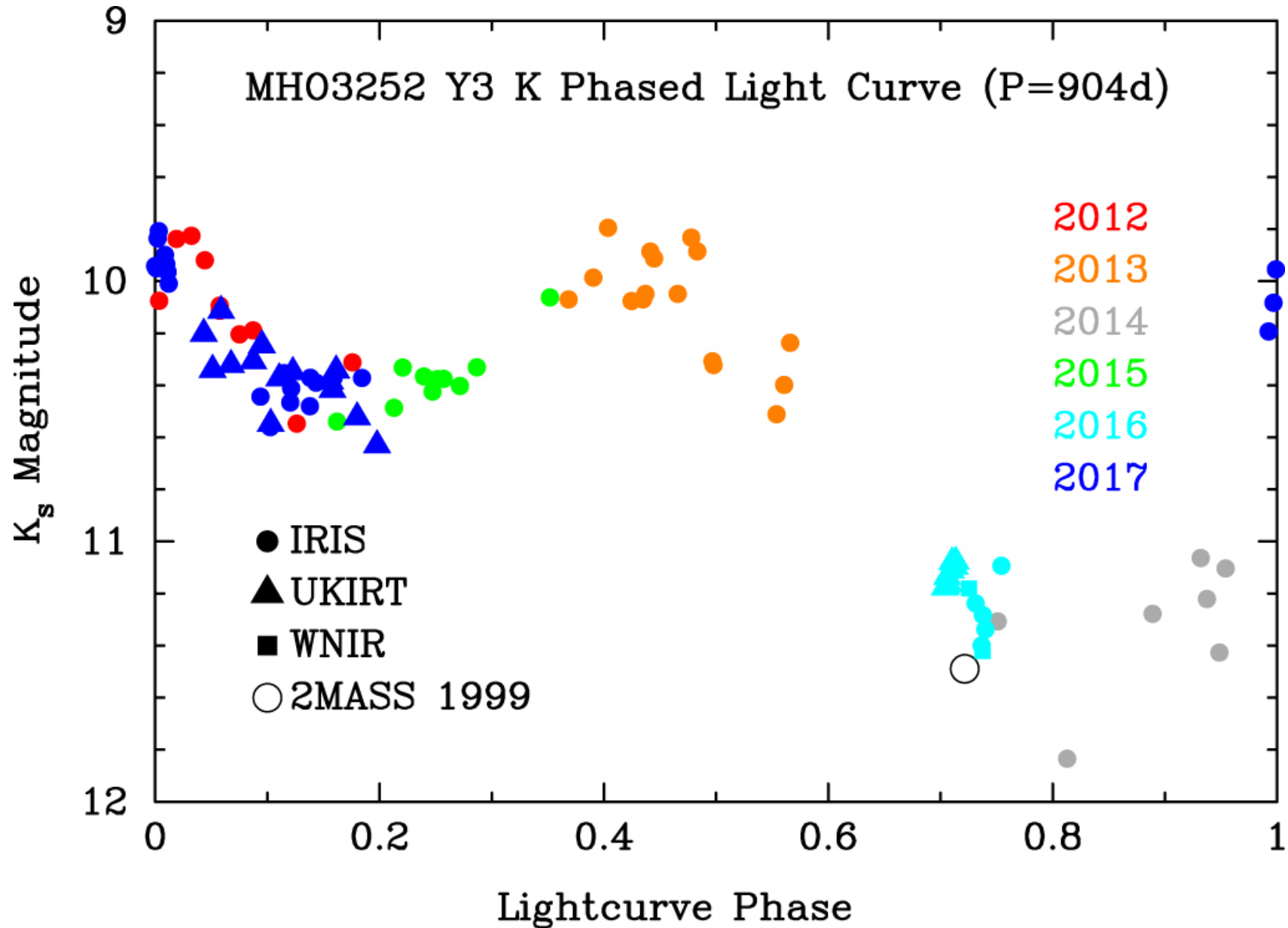
Figure 3. from Variability and Jet Activity in the YSO MHO 3252 Y3 in Serpens South null 2018 APJ 864 172 doi:10.3847/1538-4357/aad636 https://dx.doi.org/10.3847/1538-4357/aad636 © 2018. The American Astronomical Society. All rights reserved.
