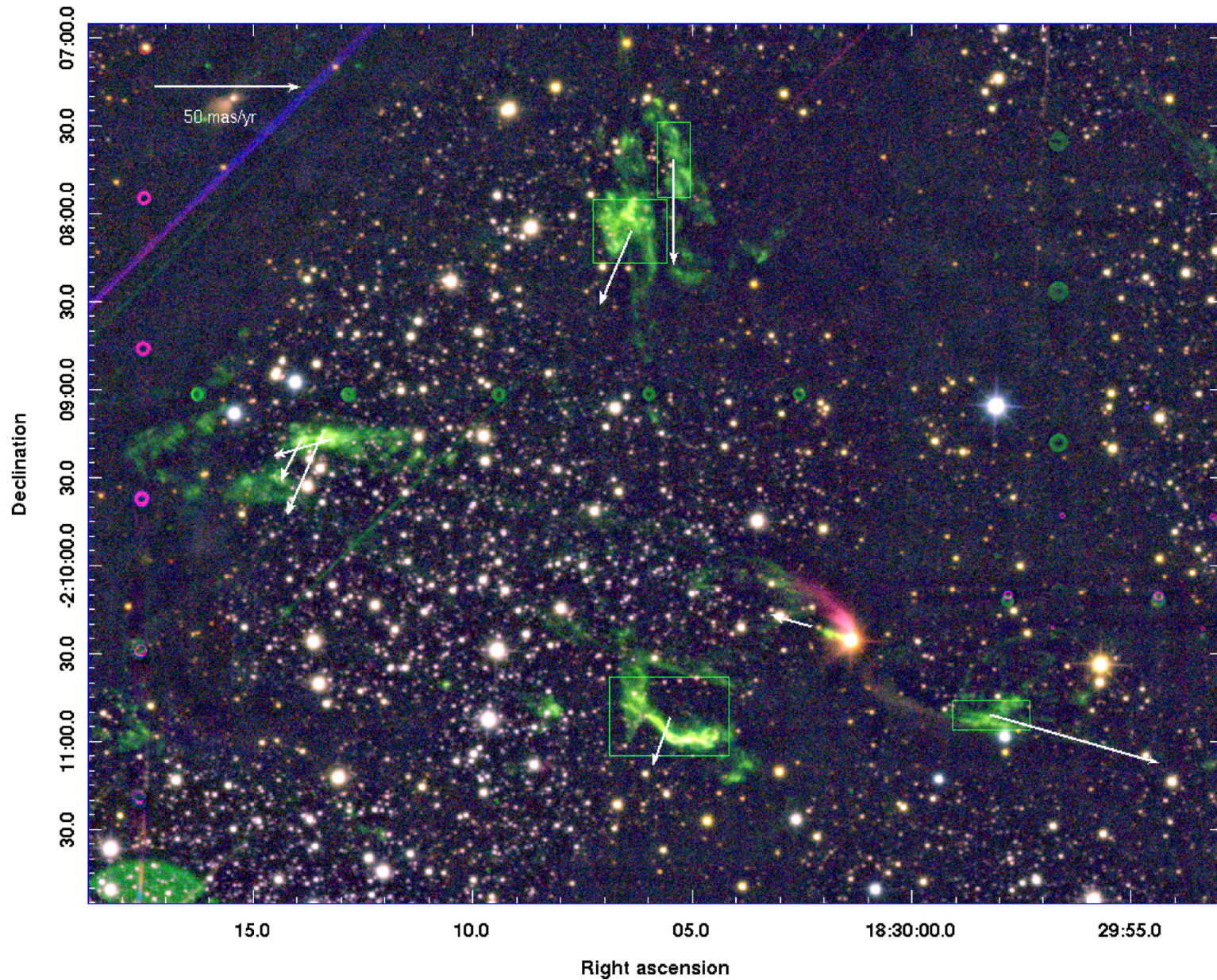
Figure 1. from Variability and Jet Activity in the YSO MHO 3252 Y3 in Serpens South null 2018 APJ 864 172 doi:10.3847/1538-4357/aad636 https://dx.doi.org/10.3847/1538-4357/aad636 © 2018. The American Astronomical Society. All rights reserved.
