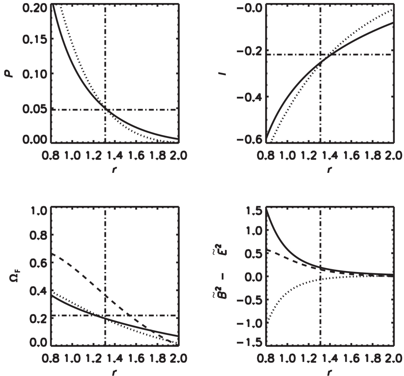
Figure 7. from Dynamic Process of Spontaneous Energy Radiation from Spinning Black Holes through Force-free Magnetic Field null 2018 APJ 864 173 doi:10.3847/1538-4357/aad4fe https://dx.doi.org/10.3847/1538-4357/aad4fe © 2018. The American Astronomical Society. All rights reserved.
