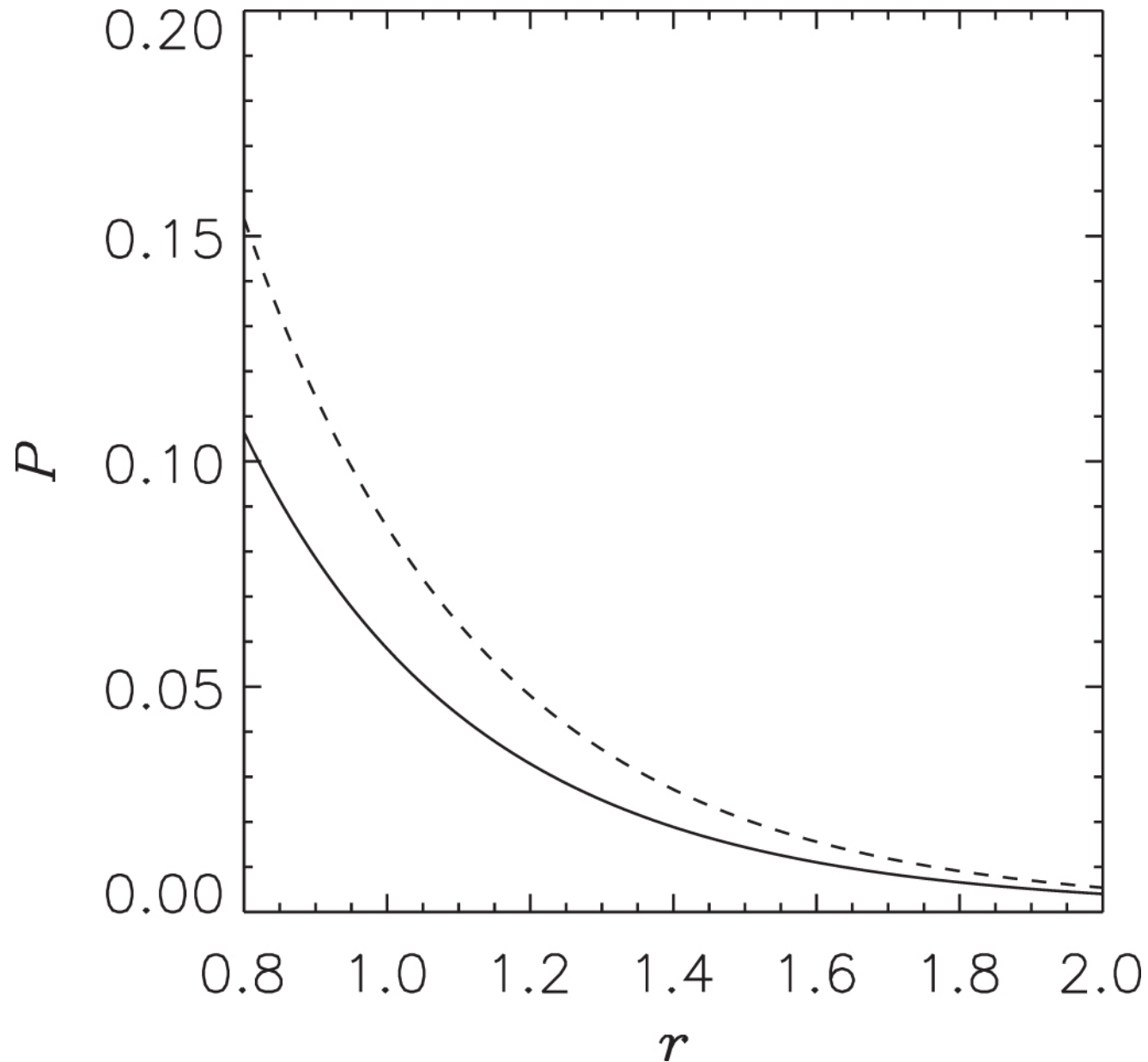
Figure 4. from Dynamic Process of Spontaneous Energy Radiation from Spinning Black Holes through Force-free Magnetic Field null 2018 APJ 864 173 doi:10.3847/1538-4357/aad4fe https://dx.doi.org/10.3847/1538-4357/aad4fe © 2018. The American Astronomical Society. All rights reserved.
