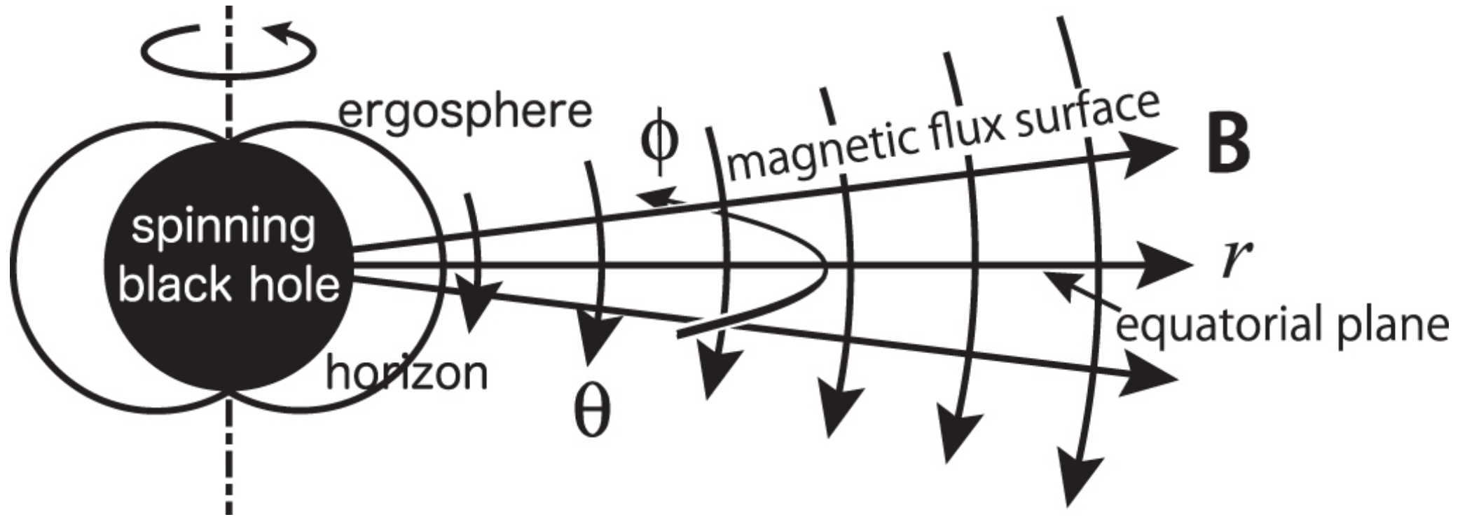
Figure 1. from Dynamic Process of Spontaneous Energy Radiation from Spinning Black Holes through Force-free Magnetic Field null 2018 APJ 864 173 doi:10.3847/1538-4357/aad4fe https://dx.doi.org/10.3847/1538-4357/aad4fe © 2018. The American Astronomical Society. All rights reserved.
