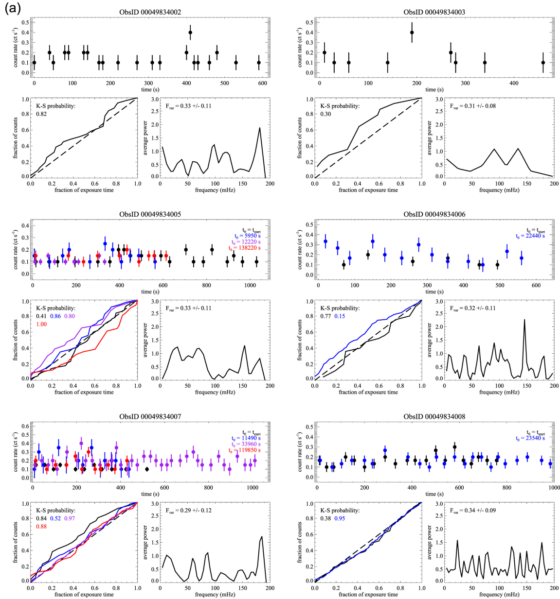
Figure 5. from No Strong Geometric Beaming in the Ultraluminous Neutron Star Binary NGC 300 ULX-1 (SN 2010da) from Swift and Gemini null 2018 APJ 863 141 doi:10.3847/1538-4357/aad3bd https://dx.doi.org/10.3847/1538-4357/aad3bd © 2018. The American Astronomical Society. All rights reserved.
