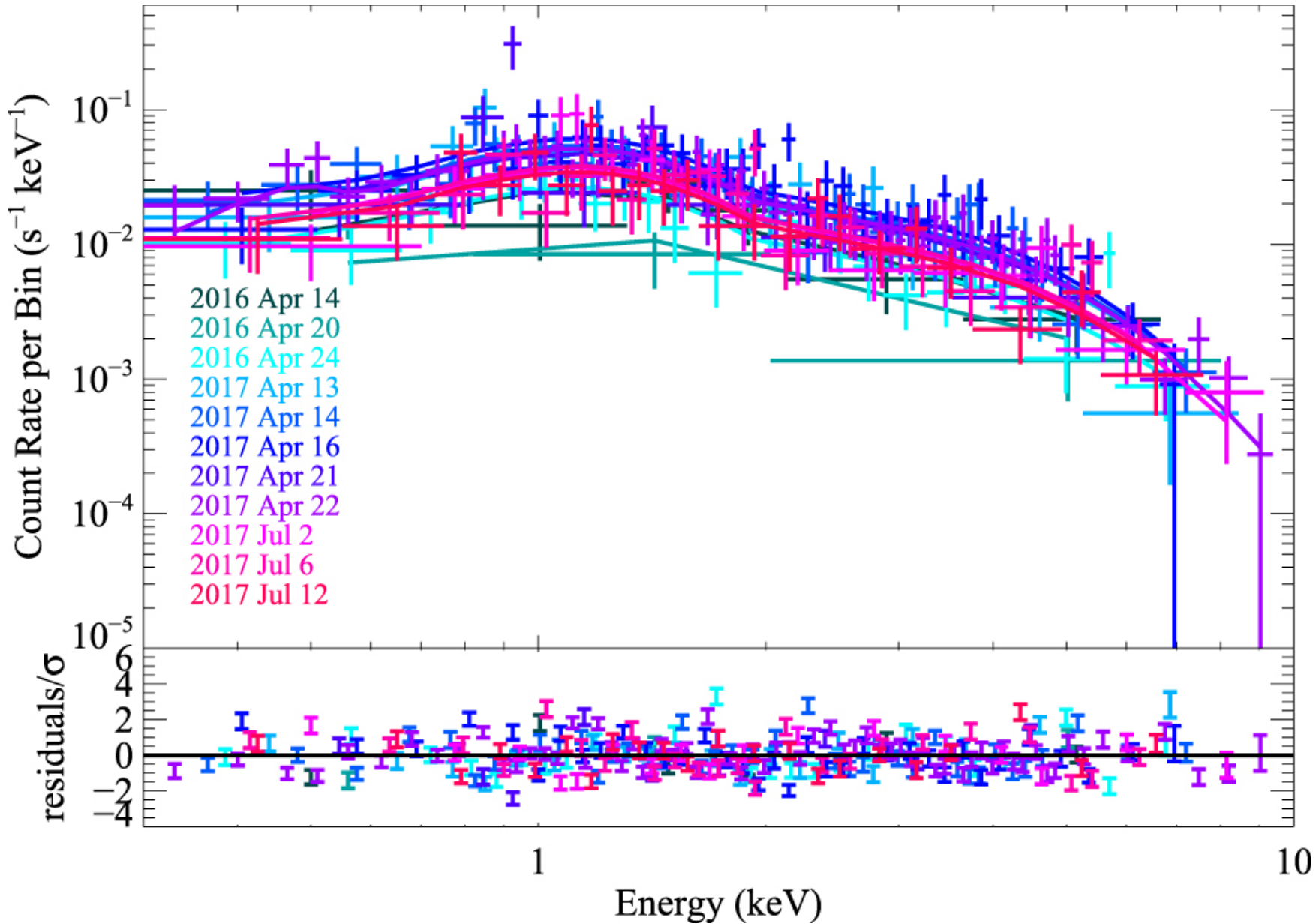
Figure 3. from No Strong Geometric Beaming in the Ultraluminous Neutron Star Binary NGC 300 ULX-1 (SN 2010da) from Swift and Gemini null 2018 APJ 863 141 doi:10.3847/1538-4357/aad3bd https://dx.doi.org/10.3847/1538-4357/aad3bd © 2018. The American Astronomical Society. All rights reserved.
