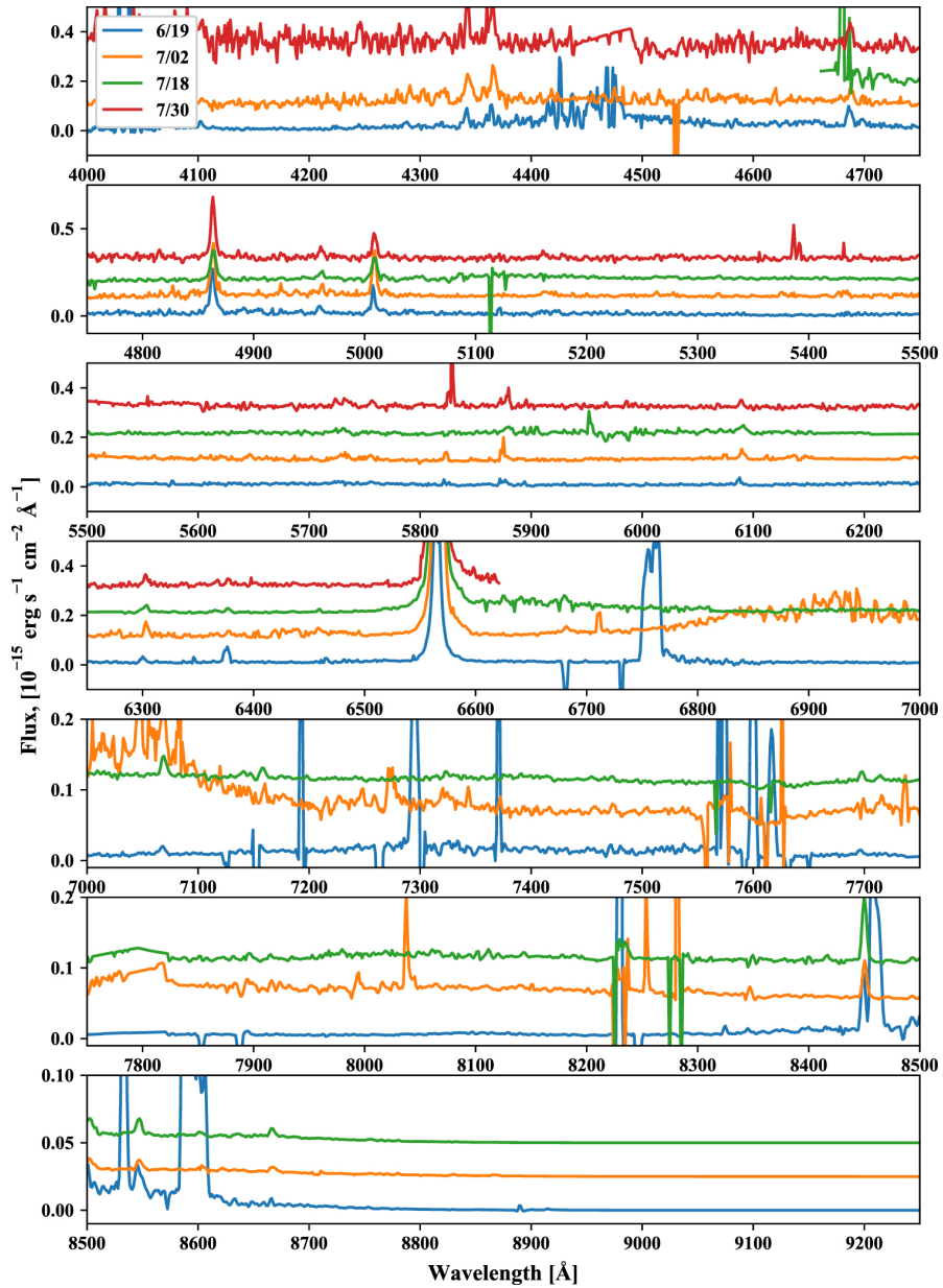
Figure 2. from No Strong Geometric Beaming in the Ultraluminous Neutron Star Binary NGC 300 ULX-1 (SN 2010da) from Swift and Gemini null 2018 APJ 863 141 doi:10.3847/1538-4357/aad3bd https://dx.doi.org/10.3847/1538-4357/aad3bd © 2018. The American Astronomical Society. All rights reserved.
