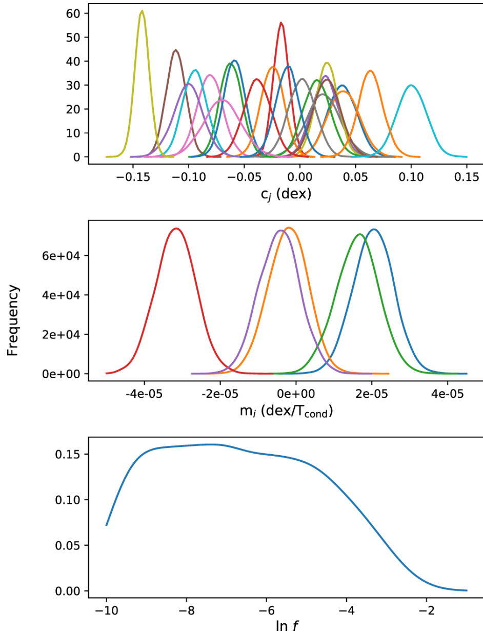
Figure 1. from Chemical Inhomogeneities in the Pleiades: Signatures of Rocky-forming Material in Stellar Atmospheres null 2018 APJ 863 179 doi:10.3847/1538-4357/aad190 https://dx.doi.org/10.3847/1538-4357/aad190
